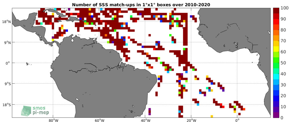
Figure 4: Number of SSS match-ups between TSG (SAMOS) SSS and the SMOS SSS L2 v662 (ESA) SSS product for the Tropical Atlantic Ocean Pi-MEP region over 1^\circ \times 1^\circ boxes and for the full satellite product period.
