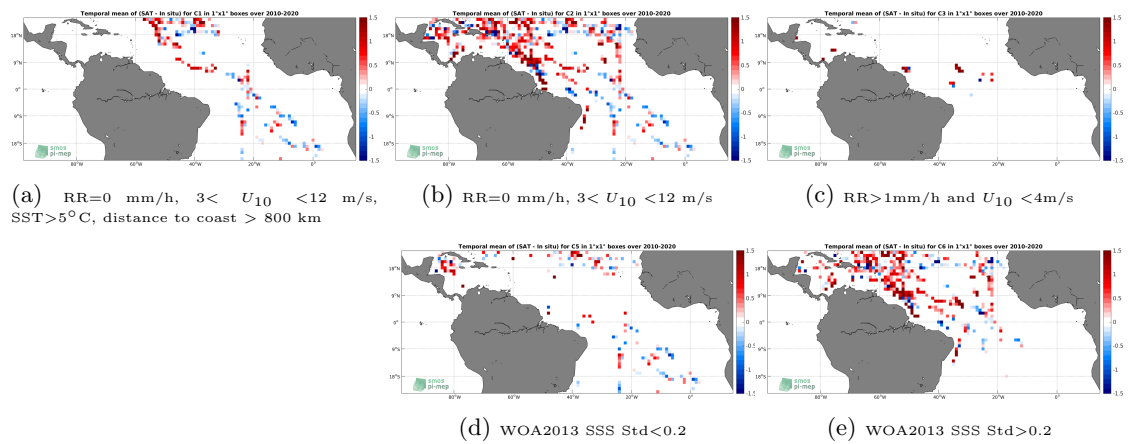
Figure 12: Temporal mean gridded over spatial boxes of size 1°x1° of \Delta SSS (SMOS SSS L2 v662 (ESA) - TSG (SAMOS)) for 5 different subdatasets corresponding to:RR=0 mm/h, 3 < U_{10} < 12 m/s, SST>5°C, distance to coast > 800 km (a), RR=0 mm/h, 3 < U_{10} < 12 m/s (b), RR>1mm/h and U_{10} < 4 m/s (c), WOA2013 SSS Std<0.2 (d), WOA2013 SSS Std>0.2 (e).
