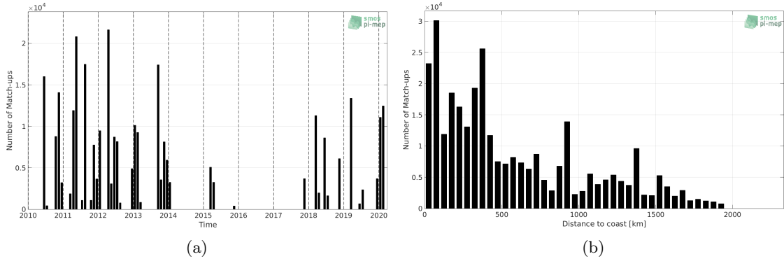
Figure 1: Number of match-ups between TSG-SAMOS and SMOS L2 v662 (ESA) SSS as a function of time (a) and as function of the distance to coast (b) over the Tropical Atlantic Ocean Pi-MEP region and for the full satellite product period.
