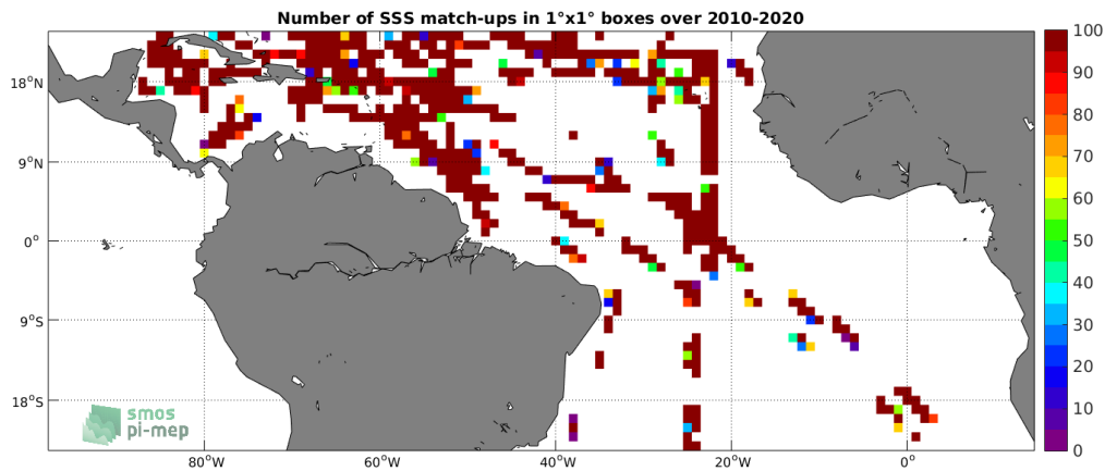
Figure 4: Number of SSS match-ups between TSG-SAMOS SSS and the SMOS L2 v662 (ESA) SSS product for the Tropical Atlantic Ocean Pi-MEP region over 1^\circ \times 1^\circ boxes and for the full satellite product period.
