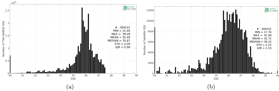
Figure 2: Histograms of SSS from TSG-SAMOS (a) and SMOS L2 v662 (ESA) (b) considering all match-up pairs per bins of 0.1 over the Tropical Atlantic Ocean Pi-MEP region and for the full satellite product period.
