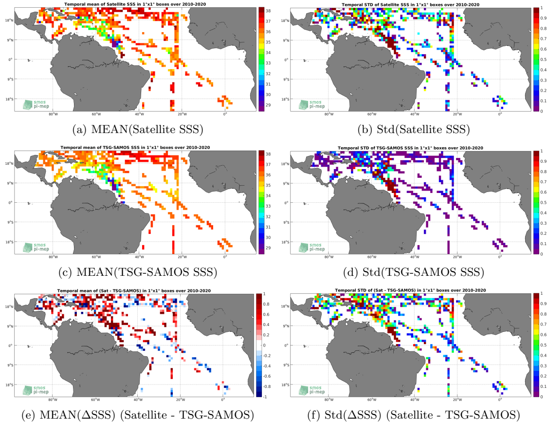
Figure 6: Temporal mean (left) and Std (right) of SSS from SMOS L2 v662 (ESA) (top), TSG-SAMOS (middle), and of \Delta SSS (Satellite - TSG-SAMOS). Only match-up pairs are used to generate these maps.
