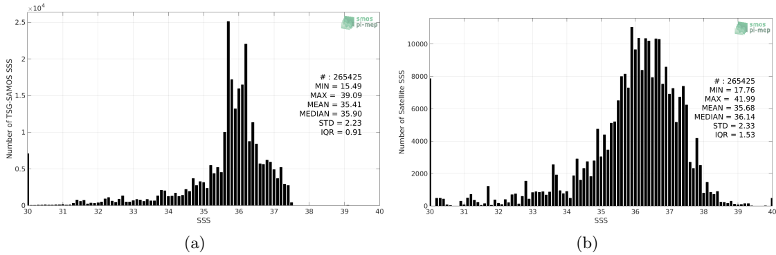
Figure 2: Histograms of SSS from TSG-SAMOS (a) and SMOS-L2-DPGS-v662 (b) considering all match-up pairs per bins of 0.1 over the Tropical Atlantic Ocean Pi-MEP region and for the full satellite product period.
