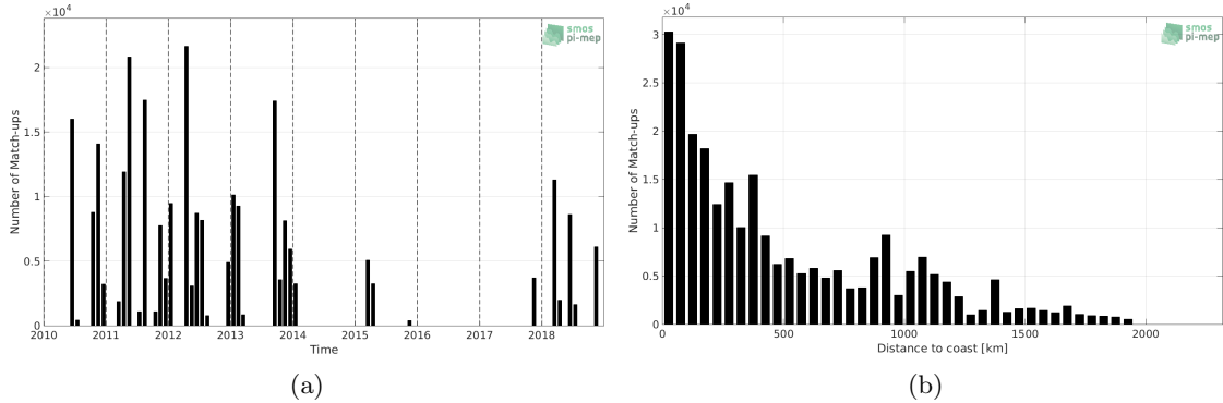
Figure 1: Number of match-ups between TSG-SAMOS and SMOS-L2-DPGS-v662 SSS as a function of time (a) and as function of the distance to coast (b) over the Tropical Atlantic Ocean Pi-MEP region and for the full satellite product period.
