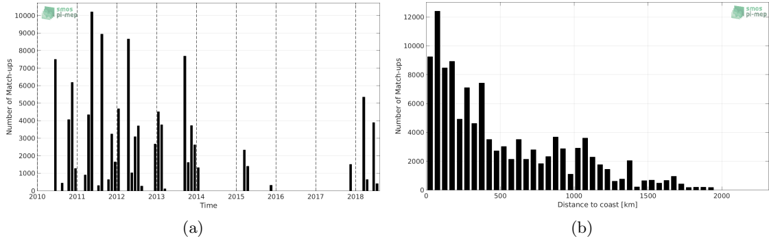
Figure 1: Number of match-ups between TSG-SAMOS and SMOS-L2-DPGS-v662 SSS as a function of time (a) and as function of the distance to coast (b) over the Tropical Atlantic Ocean Pi-MEP region and for the full satellite product period.
