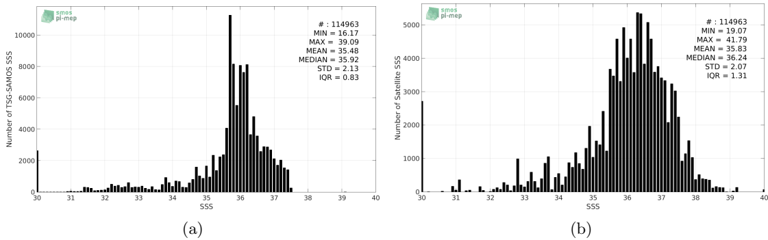
Figure 2: Histograms of SSS from TSG-SAMOS (a) and SMOS-L2-DPGS-v662 (b) considering all match-up pairs per bins of 0.1 over the Tropical Atlantic Ocean Pi-MEP region and for the full satellite product period.
