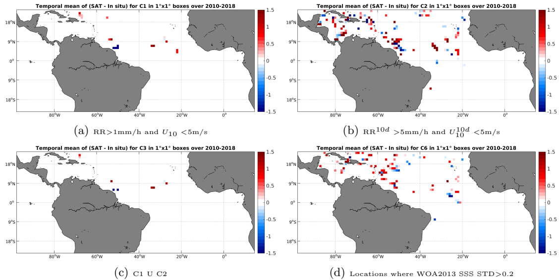
Figure 12: Temporal mean gridded over spatial boxes of size 1^\circ \times 1^\circ of \Delta SSS (SMOS-L2-DPGS-v662 - TSG-SAMOS) for 4 different subdatasets corresponding to:RR >1 mm/h and U_{10} < 5 m/s (a), RR 10d > 5 mm/h and U_{10}^{10d} < 5 m/s (b), C1 U C2 (c),Locations where WOA2013 SSS STD > 0.2 (d).
