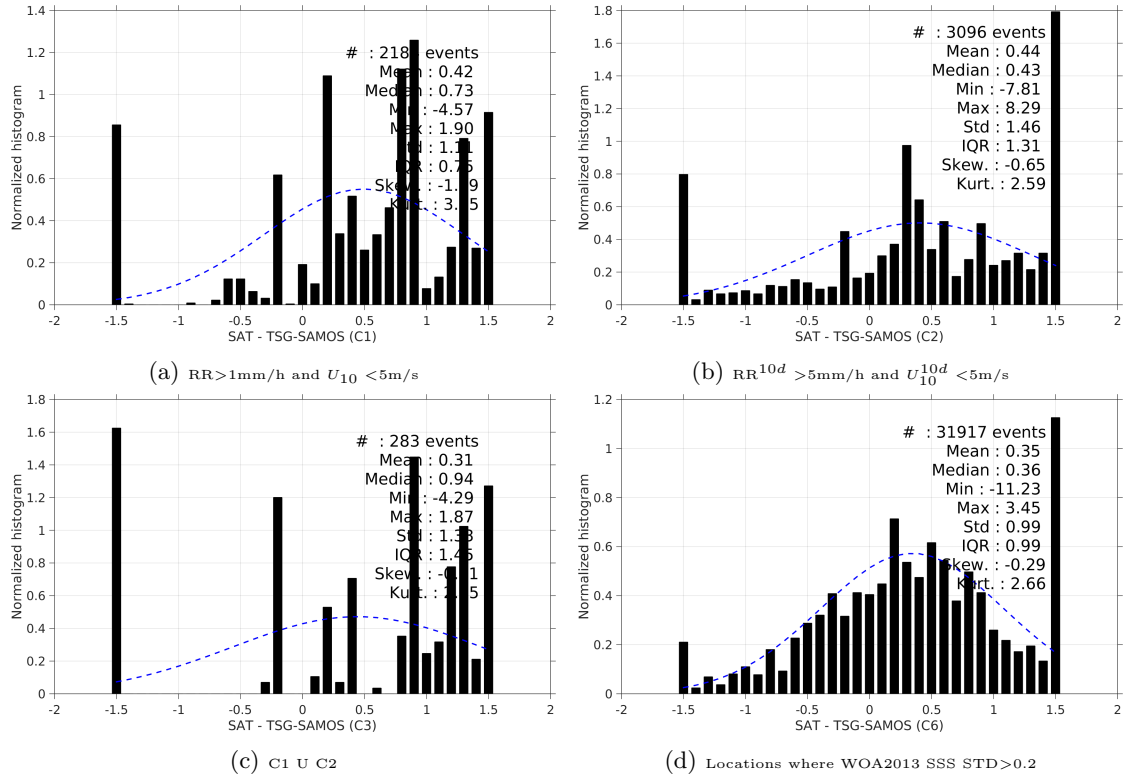
Figure 13: Normalized histogram of \Delta\text{SSS} (SMOS-L2-DPGS-v662 - TSG-SAMOS) for 6 different subdatasets corresponding to: RR > 1mm/h and U_{10} < 5\text{m/s} (a), RR^{10d} > 5\text{mm/h} and U_{10}^{10d} < 5\text{m/s} (b), C1 U C2 (c), Locations where WOA2013 SSS STD > 0.2 (d).
