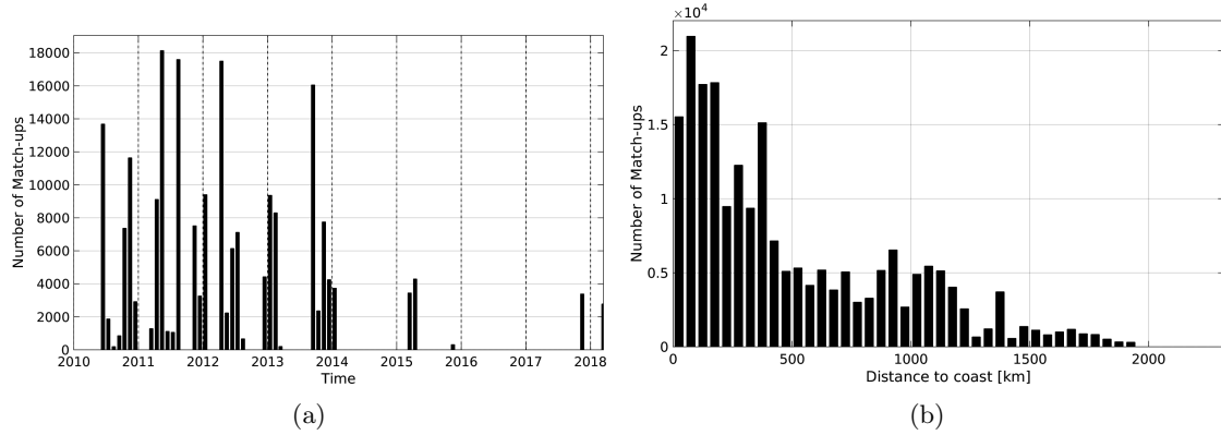
Figure 1: Number of match-ups between TSG-SAMOS and SMOS-L2-DPGS-v662 SSS as a function of time (a) and as function of the distance to coast (b) over the Tropical Atlantic Ocean Pi-MEP region and for the full satellite product period.
