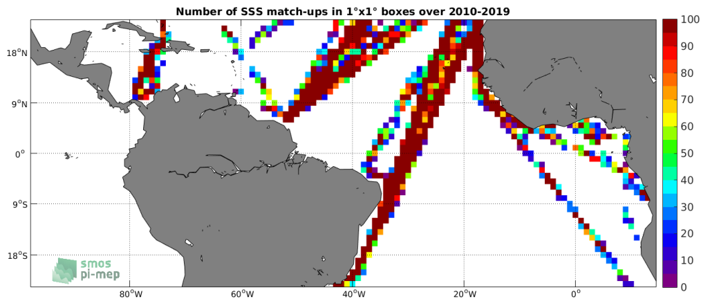
Figure 4: Number of SSS match-ups between TSG (LEGOS-DM) SSS and the SMOS SSS L2 v662 (ESA) SSS product for the Tropical Atlantic Ocean Pi-MEP region over 1^\circ \times 1^\circ boxes and for the full satellite product period.
