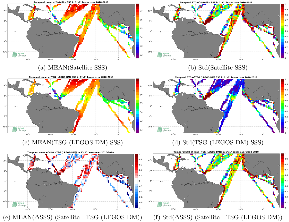
Figure 6: Temporal mean (left) and Std (right) of SSS from SMOS SSS L2 v662 (ESA) (top), TSG (LEGOS-DM) (middle), and of \Delta SSS (Satellite - TSG (LEGOS-DM)). Only match-up pairs are used to generate these maps.
