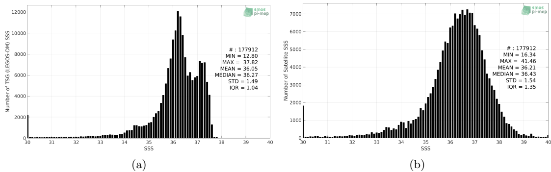
Figure 2: Histograms of SSS from TSG (LEGOS-DM) (a) and SMOS SSS L2 v662 (ESA) (b) considering all match-up pairs per bins of 0.1 over the Tropical Atlantic Ocean Pi-MEP region and for the full satellite product period.
