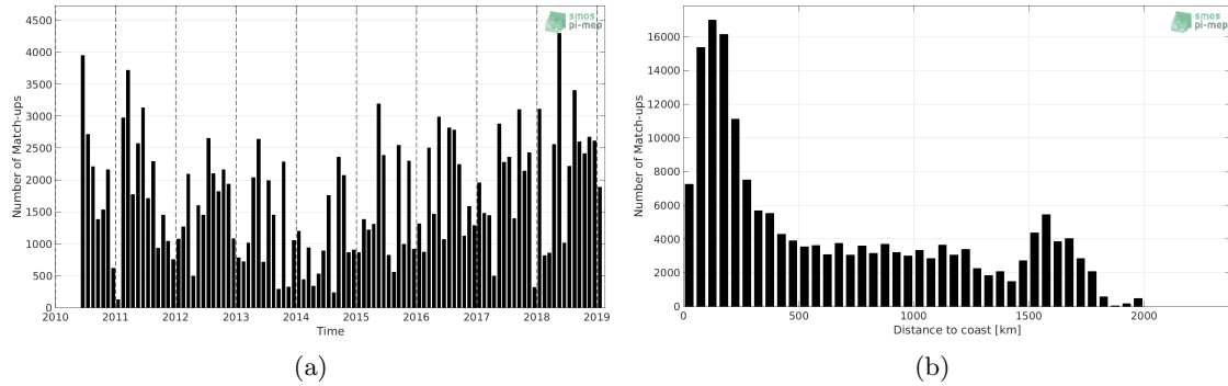
Figure 1: Number of match-ups between TSG (LEGOS-DM) and SMOS SSS L2 v662 (ESA) SSS as a function of time (a) and as function of the distance to coast (b) over the Tropical Atlantic Ocean Pi-MEP region and for the full satellite product period.
