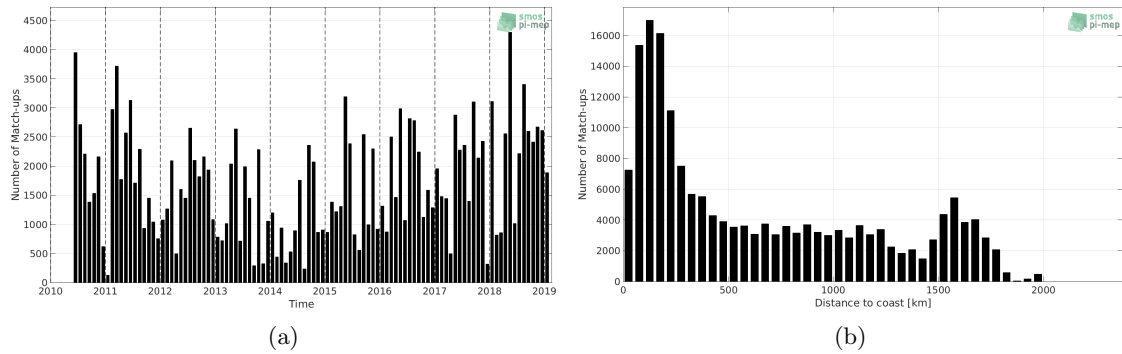
Figure 1: Number of match-ups between TSG-LEGOS-DM and SMOS L2 v662 (ESA) SSS as a function of time (a) and as function of the distance to coast (b) over the Tropical Atlantic Ocean Pi-MEP region and for the full satellite product period.
