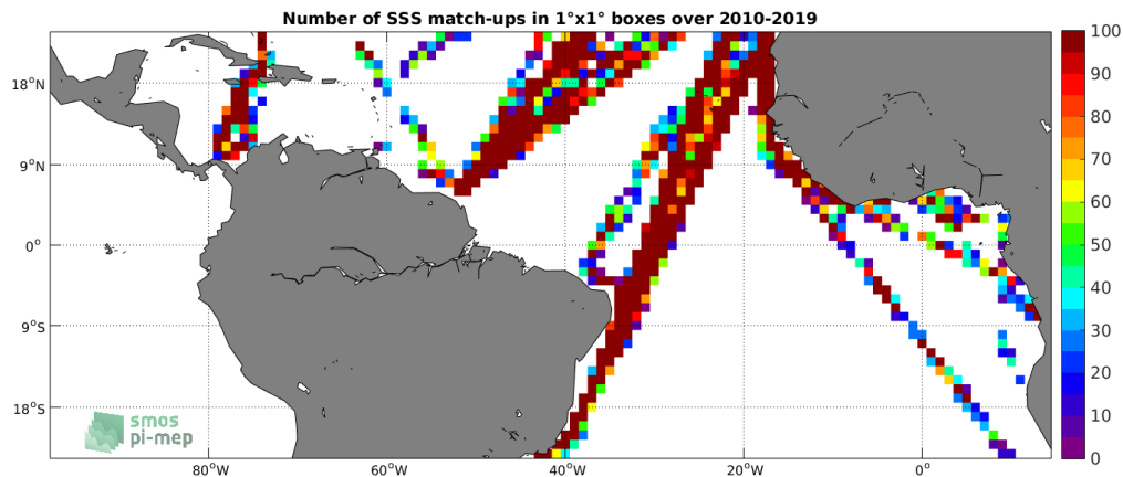
Figure 4: Number of SSS match-ups between TSG-LEGOS-DM SSS and the SMOS L2 v662 (ESA) SSS product for the Tropical Atlantic Ocean Pi-MEP region over 1^\circ \times 1^\circ boxes and for the full satellite product period.
