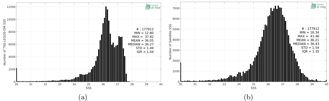
Figure 2: Histograms of SSS from TSG-LEGOS-DM (a) and SMOS L2 v662 (ESA) (b) considering all match-up pairs per bins of 0.1 over the Tropical Atlantic Ocean Pi-MEP region and for the full satellite product period.
