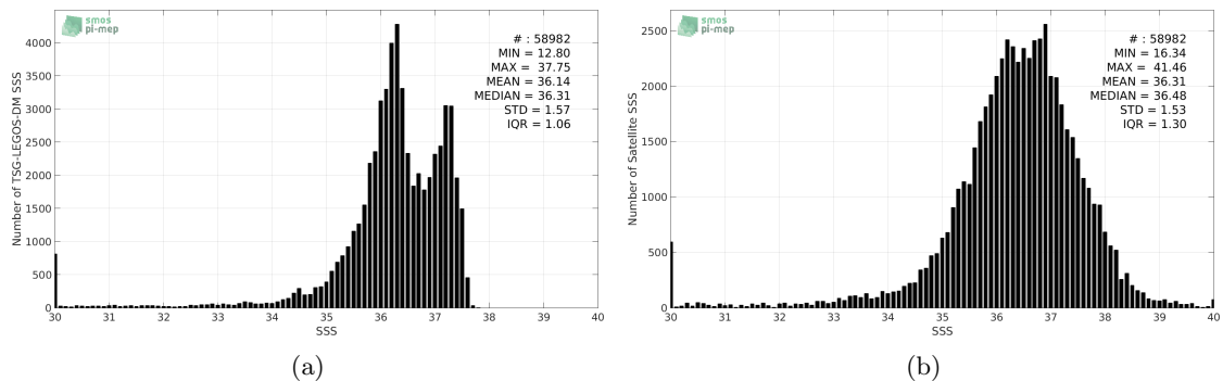
Figure 2: Histograms of SSS from TSG-LEGOS-DM (a) and SMOS-L2-DPGS-v662 (b) considering all match-up pairs per bins of 0.1 over the Tropical Atlantic Ocean Pi-MEP region and for the full satellite product period.
