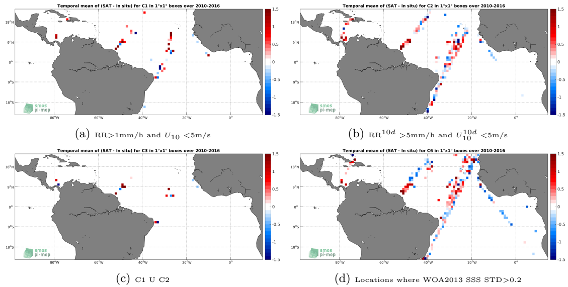
Figure 12: Temporal mean gridded over spatial boxes of size 1^\circ \times 1^\circ of \Delta SSS (SMOS-L2-DPGS-v662 - TSG-LEGOS-DM) for 4 different subdatasets corresponding to: RR > 1\text{mm/h} and U_{10} < 5\text{m/s} (a), RR^{10d} > 5\text{mm/h} and U_{10}^{10d} < 5\text{m/s} (b), C1 U C2 (c), Locations where WOA2013 SSS STD > 0.2 (d).
