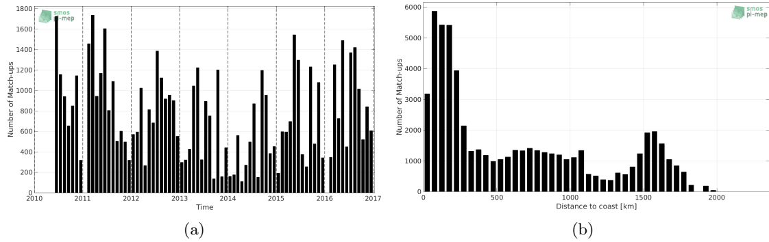
Figure 1: Number of match-ups between TSG-LEGOS-DM and SMOS-L2-DPGS-v662 SSS as a function of time (a) and as function of the distance to coast (b) over the Tropical Atlantic Ocean Pi-MEP region and for the full satellite product period.
