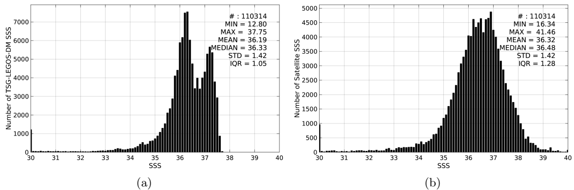
Figure 2: Histograms of SSS from TSG-LEGOS-DM (a) and SMOS-L2-DPGS-v662 (b) considering all match-up pairs per bins of 0.1 over the Tropical Atlantic Ocean Pi-MEP region and for the full satellite product period.
