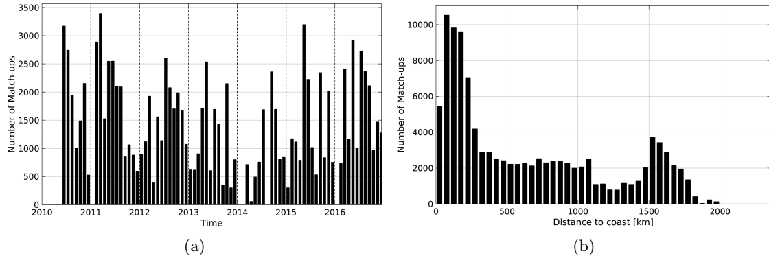
Figure 1: Number of match-ups between TSG-LEGOS-DM and SMOS-L2-DPGS-v662 SSS as a function of time (a) and as function of the distance to coast (b) over the Tropical Atlantic Ocean Pi-MEP region and for the full satellite product period.
