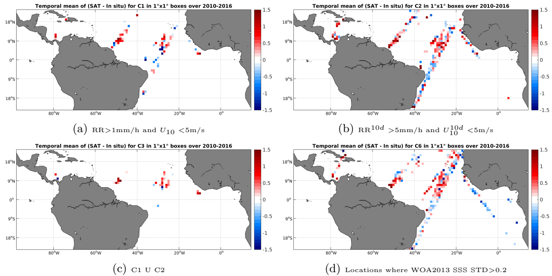
Figure 12: Temporal mean gridded over spatial boxes of size 1^\circ \times 1^\circ of \Delta SSS (SMOS-L2-DPGS-v662 - TSG-LEGOS-DM) for 4 different subdatasets corresponding to:RR>1mm/h and U_{10} < 5\text{m/s} (a), RR^{10d} > 5\text{mm/h} and U_{10}^{10d} < 5\text{m/s} (b), C1 U C2 (c),Locations where WOA2013 SSS STD>0.2 (d).
