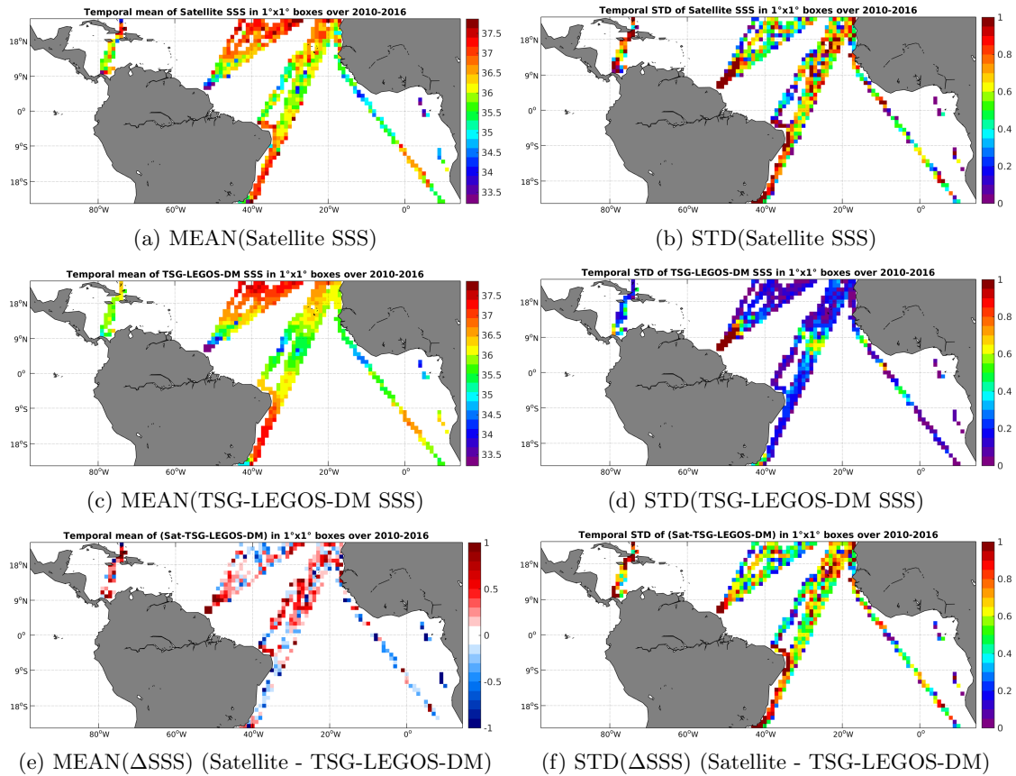
Figure 6: Temporal mean (left) and STD (right) of SSS from SMOS-L2-DPGS-v662 (top), TSG-LEGOS-DM (middle), and of \Delta SSS (Satellite - TSG-LEGOS-DM). Only match-up pairs are used to generate these maps.
