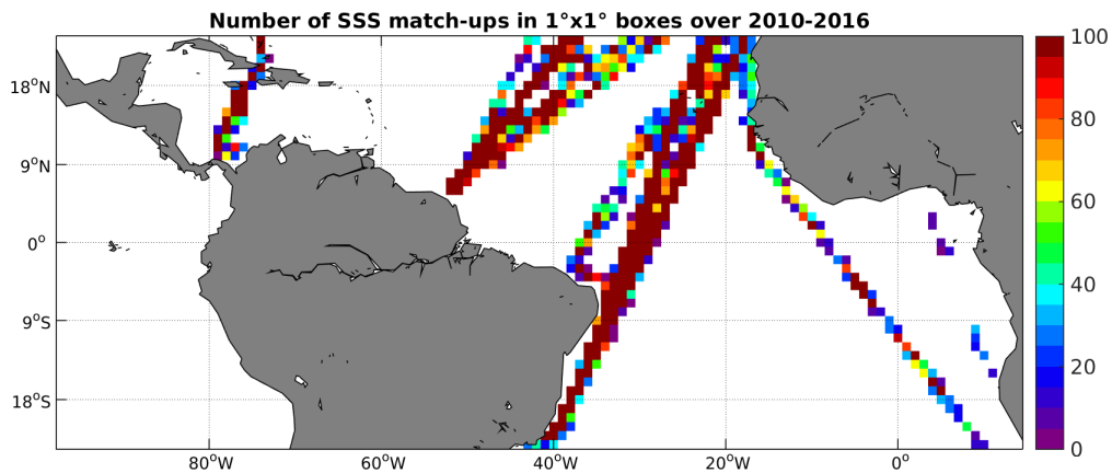
Figure 4: Number of SSS match-ups between TSG-LEGOS-DM SSS and the SMOS-L2-DPGS-v662 SSS product for the Tropical Atlantic Ocean Pi-MEP region over 1^\circ \times 1^\circ boxes and for the full satellite product period.
