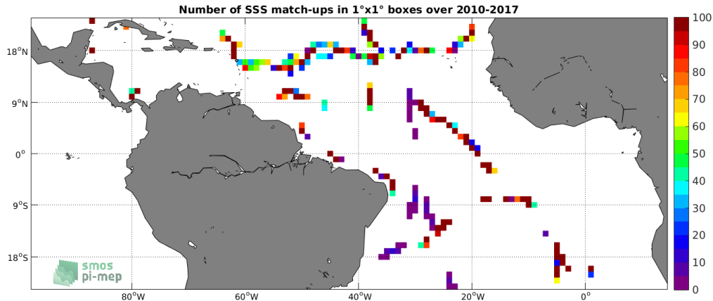
Figure 4: Number of SSS match-ups between TSG (GOSUD-Sailing-ship) SSS and the SMOS SSS L2 v662 (ESA) SSS product for the Tropical Atlantic Ocean Pi-MEP region over 1^\circ \times 1^\circ boxes and for the full satellite product period.
