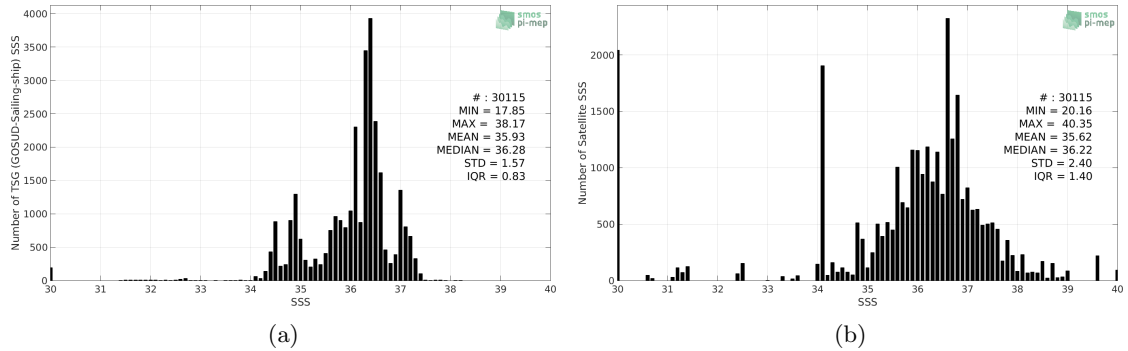
Figure 2: Histograms of SSS from TSG (GOSUD-Sailing-ship) (a) and SMOS SSS L2 v662 (ESA) (b) considering all match-up pairs per bins of 0.1 over the Tropical Atlantic Ocean Pi-MEP region and for the full satellite product period.
