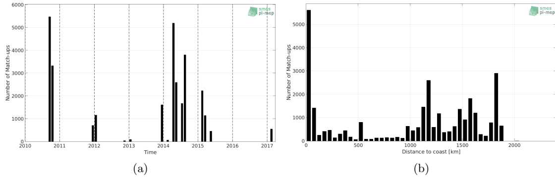
Figure 1: Number of match-ups between TSG (GOSUD-Sailing-ship) and SMOS SSS L2 v662 (ESA) SSS as a function of time (a) and as function of the distance to coast (b) over the Tropical Atlantic Ocean Pi-MEP region and for the full satellite product period.
