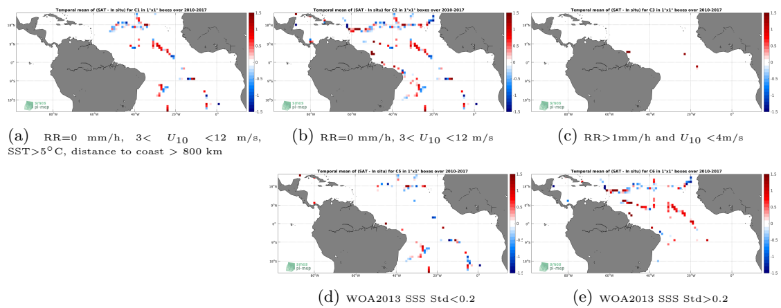
Figure 12: Temporal mean gridded over spatial boxes of size 1°x1° of \Delta SSS (SMOS SSS L2 v662 (ESA) - TSG (GOSUD-Sailing-ship)) for 5 different subdatasets corresponding to:RR=0 mm/h, 3 < U_{10} < 12 m/s, SST>5°C, distance to coast > 800 km (a), RR=0 mm/h, 3 < U_{10} < 12 m/s (b), RR>1mm/h and U_{10} < 4 m/s (c), WOA2013 SSS Std<0.2 (d), WOA2013 SSS Std>0.2 (e).
