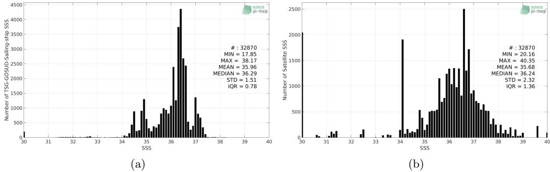
Figure 2: Histograms of SSS from TSG-GOSUD-Sailing-ship (a) and SMOS L2 v662 (ESA) (b) considering all match-up pairs per bins of 0.1 over the Tropical Atlantic Ocean Pi-MEP region and for the full satellite product period.
