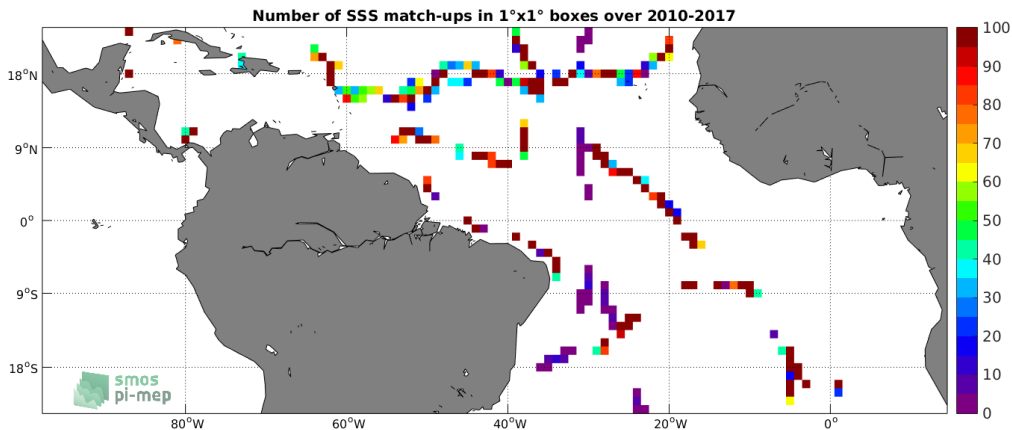
Figure 4: Number of SSS match-ups between TSG-GOSUD-Sailing-ship SSS and the SMOS L2 v662 (ESA) SSS product for the Tropical Atlantic Ocean Pi-MEP region over 1°x1° boxes and for the full satellite product period.
