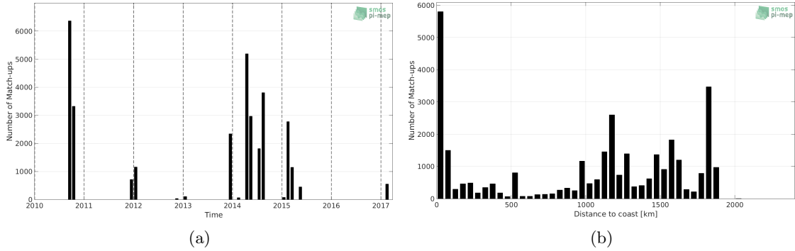
Figure 1: Number of match-ups between TSG-GOSUD-Sailing-ship and SMOS L2 v662 (ESA) SSS as a function of time (a) and as function of the distance to coast (b) over the Tropical Atlantic Ocean Pi-MEP region and for the full satellite product period.
