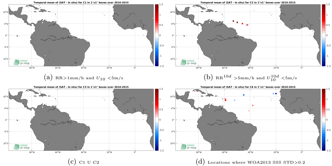
Figure 12: Temporal mean gridded over spatial boxes of size 1^\circ \times 1^\circ of \Delta\text{SSS} (SMOS-L2-DPGS-v662 - TSG-GOSUD-Sailing-ship) for 4 different subdatasets corresponding to: \text{RR} > 1\text{mm/h} and U_{10} < 5\text{m/s} (a), \text{RR}^{10d} > 5\text{mm/h} and U_{10}^{10d} < 5\text{m/s} (b), C1 U C2 (c), Locations where WOA2013 SSS STD > 0.2 (d).
