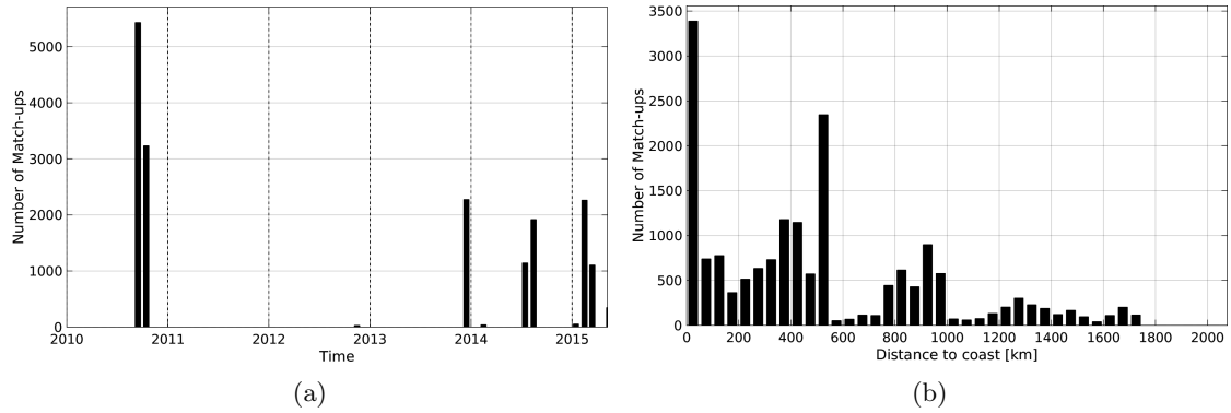
Figure 1: Number of match-ups between TSG-GOSUD-Sailing-ship and SMOS-L2-DPGS-v662 SSS as a function of time (a) and as function of the distance to coast (b) over the Tropical Atlantic Ocean Pi-MEP region and for the full satellite product period.
