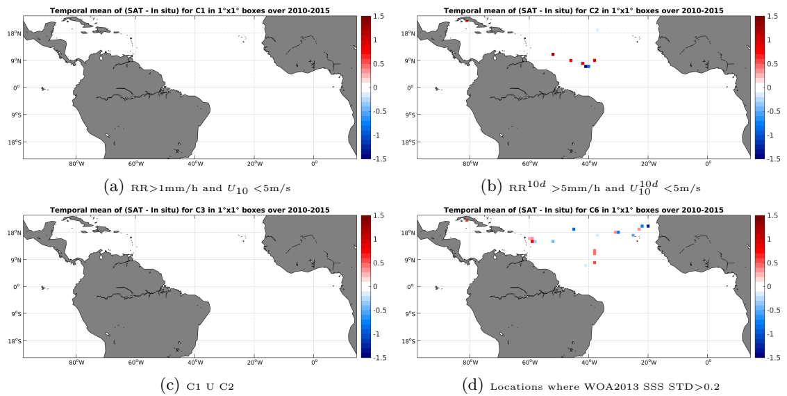
Figure 12: Temporal mean gridded over spatial boxes of size 1^\circ \times 1^\circ of \Delta SSS (SMOS-L2-DPGS-v662 - TSG-GOSUD-Sailing-ship) for 4 different subdatasets corresponding to:RR >1 mm/h and U_{10} < 5 m/s (a), RR^{10d} > 5 mm/h and U_{10}^{10d} < 5 m/s (b), C1 U C2 (c),Locations where WOA2013 SSS STD >0.2 (d).
