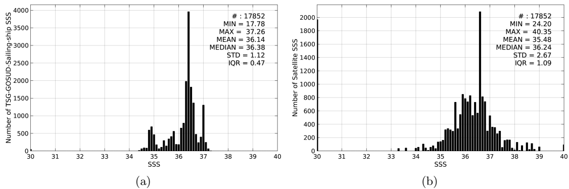
Figure 2: Histograms of SSS from TSG-GOSUD-Sailing-ship (a) and SMOS-L2-DPGS-v662 (b) considering all match-up pairs per bins of 0.1 over the Tropical Atlantic Ocean Pi-MEP region and for the full satellite product period.
