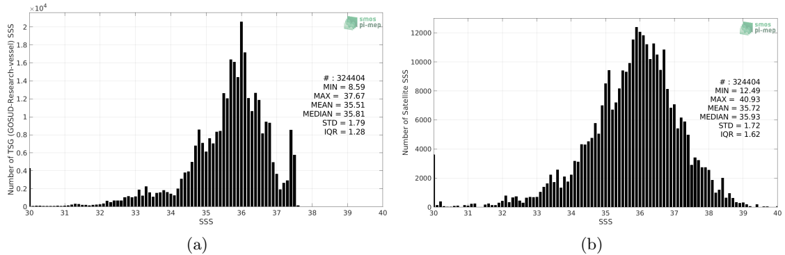
Figure 2: Histograms of SSS from TSG (GOSUD-Research-vessel) (a) and SMOS SSS L2 v662 (ESA) (b) considering all match-up pairs per bins of 0.1 over the Tropical Atlantic Ocean Pi-MEP region and for the full satellite product period.
