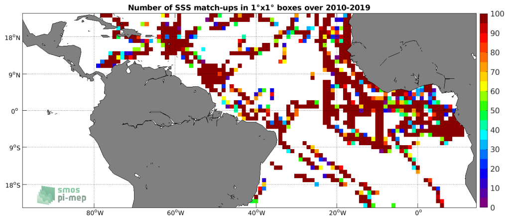
Figure 4: Number of SSS match-ups between TSG (GOSUD-Research-vessel) SSS and the SMOS SSS L2 v662 (ESA) SSS product for the Tropical Atlantic Ocean Pi-MEP region over 1^\circ \times 1^\circ boxes and for the full satellite product period.
