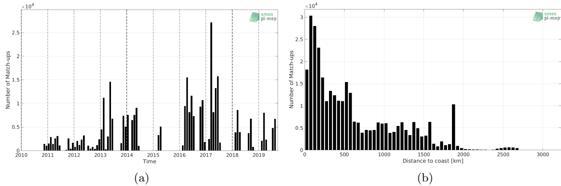
Figure 1: Number of match-ups between TSG (GOSUD-Research-vessel) and SMOS SSS L2 v662 (ESA) SSS as a function of time (a) and as function of the distance to coast (b) over the Tropical Atlantic Ocean Pi-MEP region and for the full satellite product period.
