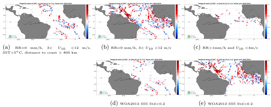
Figure 12: Temporal mean gridded over spatial boxes of size 1°x1° of \Delta SSS (SMOS SSS L2 v662 (ESA) - TSG (GOSUD-Research-vessel)) for 5 different subdatasets corresponding to:RR=0 mm/h, 3 < U_{10} < 12 m/s, SST>5°C, distance to coast > 800 km (a), RR=0 mm/h, 3 < U_{10} < 12 m/s (b), RR>1mm/h and U_{10} < 4 m/s (c), WOA2013 SSS Std<0.2 (d), WOA2013 SSS Std>0.2 (e).
