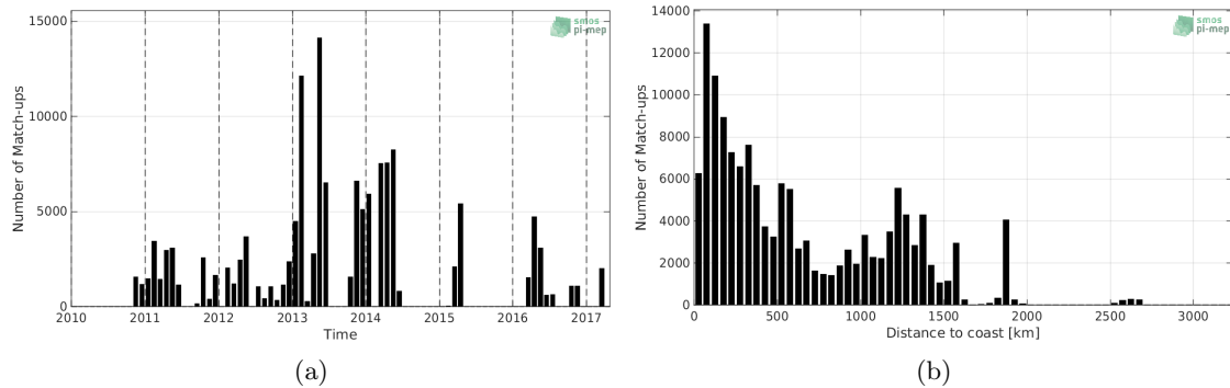
Figure 1: Number of match-ups between TSG-GOSUD-Research-vessel and SMOS-L2-DPGS-v662 SSS as a function of time (a) and as function of the distance to coast (b) over the Tropical Atlantic Ocean Pi-MEP region and for the full satellite product period.
