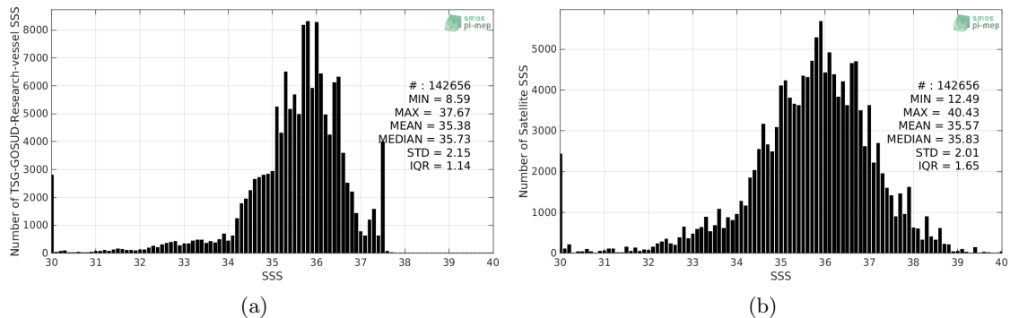
Figure 2: Histograms of SSS from TSG-GOSUD-Research-vessel (a) and SMOS-L2-DPGS-v662 (b) considering all match-up pairs per bins of 0.1 over the Tropical Atlantic Ocean Pi-MEP region and for the full satellite product period.
