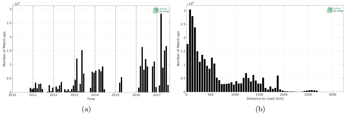
Figure 1: Number of match-ups between TSG-GOSUD-Research-vessel and SMOS-L2-DPGS-v662 SSS as a function of time (a) and as function of the distance to coast (b) over the Tropical Atlantic Ocean Pi-MEP region and for the full satellite product period.
