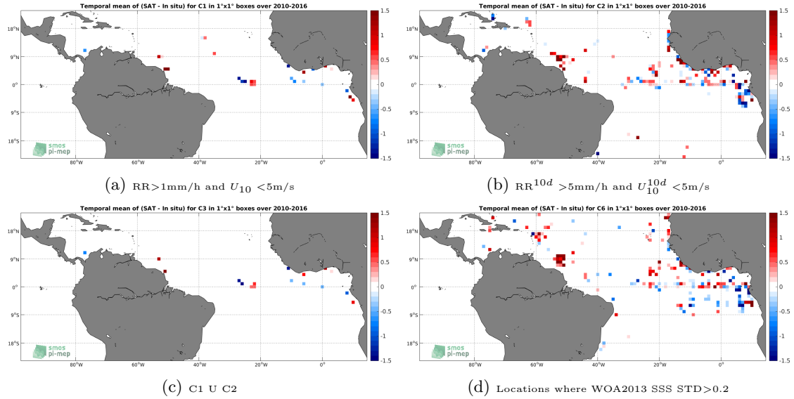
Figure 12: Temporal mean gridded over spatial boxes of size 1^\circ \times 1^\circ of \Delta SSS (SMOS-L2-DPGS-v662 - TSG-GOSUD-Research-vessel) for 4 different subdatasets corresponding to: RR > 1mm/h and U_{10} < 5\text{m/s} (a), RR^{10d} > 5\text{mm/h} and U_{10}^{10d} < 5\text{m/s} (b), C1 U C2 (c), Locations where WOA2013 SSS STD > 0.2 (d).
