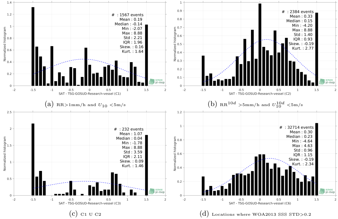
Figure 13: Normalized histogram of \Delta SSS (SMOS-L2-DPGS-v662 - TSG-GOSUD-Research-vessel) for 6 different subdatasets corresponding to: RR > 1mm/h and U_{10} < 5 m/s (a), RR^{10d} > 5 mm/h and U_{10}^{10d} < 5 m/s (b), C1 U C2 (c), Locations where WOA2013 SSS STD > 0.2 (d).
