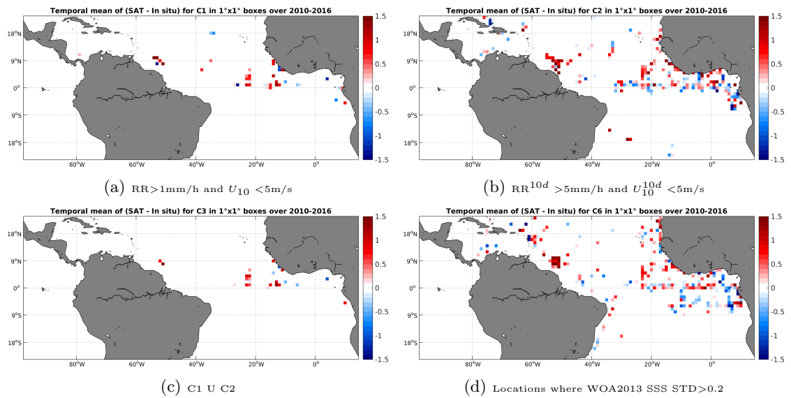
Figure 12: Temporal mean gridded over spatial boxes of size 1^\circ \times 1^\circ of \Delta SSS (SMOS-L2-DPGS-v662 - TSG-GOSUD-Research-vessel) for 4 different subdatasets corresponding to:RR >1 mm/h and U_{10} < 5 m/s (a), RR^{10d} > 5 mm/h and U_{10}^{10d} < 5 m/s (b), C1 U C2 (c),Locations where WOA2013 SSS STD >0.2 (d).
