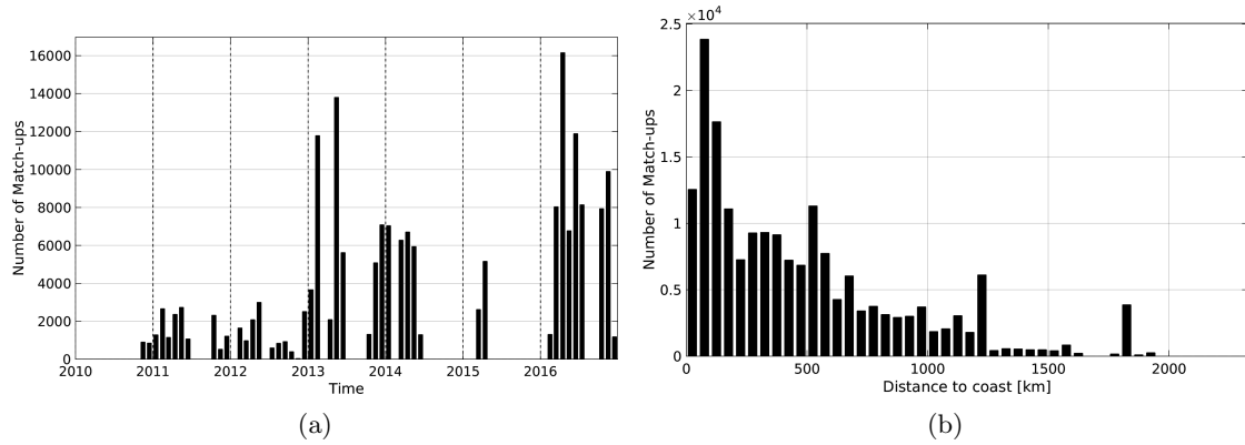
Figure 1: Number of match-ups between TSG-GOSUD-Research-vessel and SMOS-L2-DPGS-v662 SSS as a function of time (a) and as function of the distance to coast (b) over the Tropical Atlantic Ocean Pi-MEP region and for the full satellite product period.
