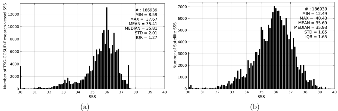
Figure 2: Histograms of SSS from TSG-GOSUD-Research-vessel (a) and SMOS-L2-DPGS-v662 (b) considering all match-up pairs per bins of 0.1 over the Tropical Atlantic Ocean Pi-MEP region and for the full satellite product period.
