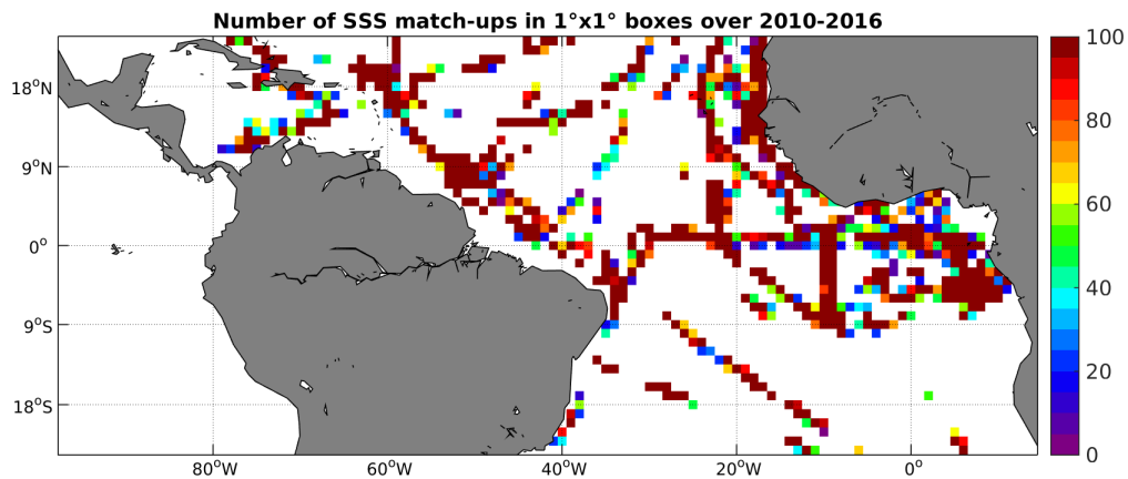
Figure 4: Number of SSS match-ups between TSG-GOSUD-Research-vessel SSS and the SMOS-L2-DPGS-v662 SSS product for the Tropical Atlantic Ocean Pi-MEP region over 1^\circ \times 1^\circ boxes and for the full satellite product period.
