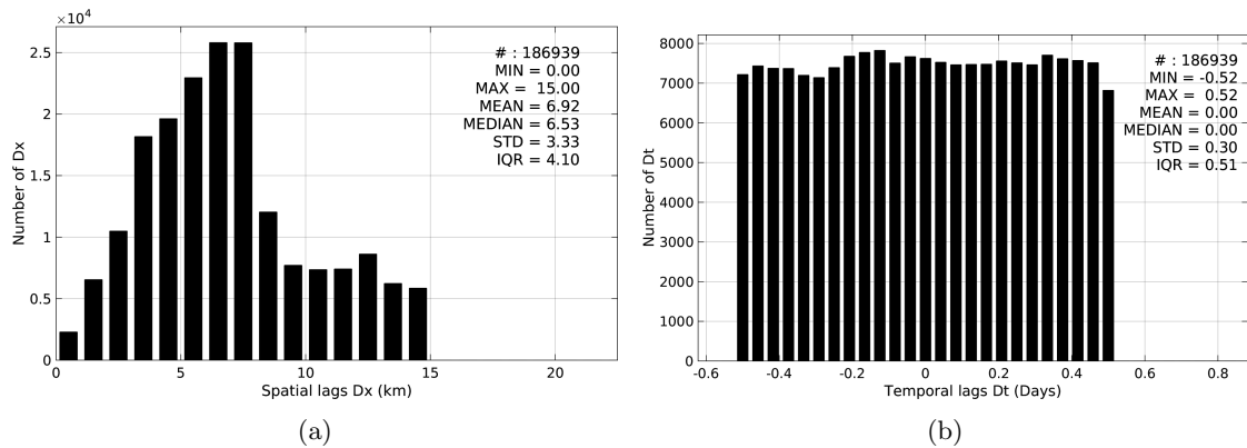
Figure 5: Histograms of the spatial (a) and temporal (b) lags between the time of the TSG-GOSUD-Research-vessel measurements and the date of the corresponding SMOS-L2-DPGS-v662 SSS product.
