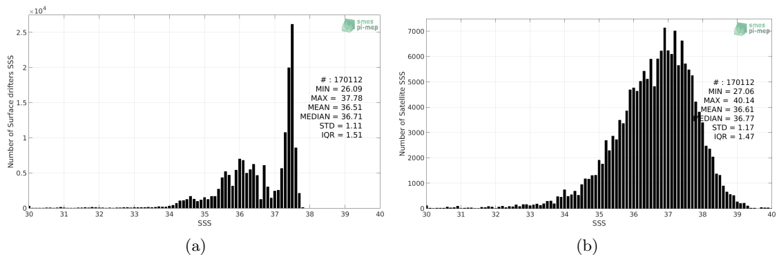
Figure 2: Histograms of SSS from Surface drifters (a) and SMOS SSS L2 v662 (ESA) (b) considering all match-up pairs per bins of 0.1 over the Tropical Atlantic Ocean Pi-MEP region and for the full satellite product period.
