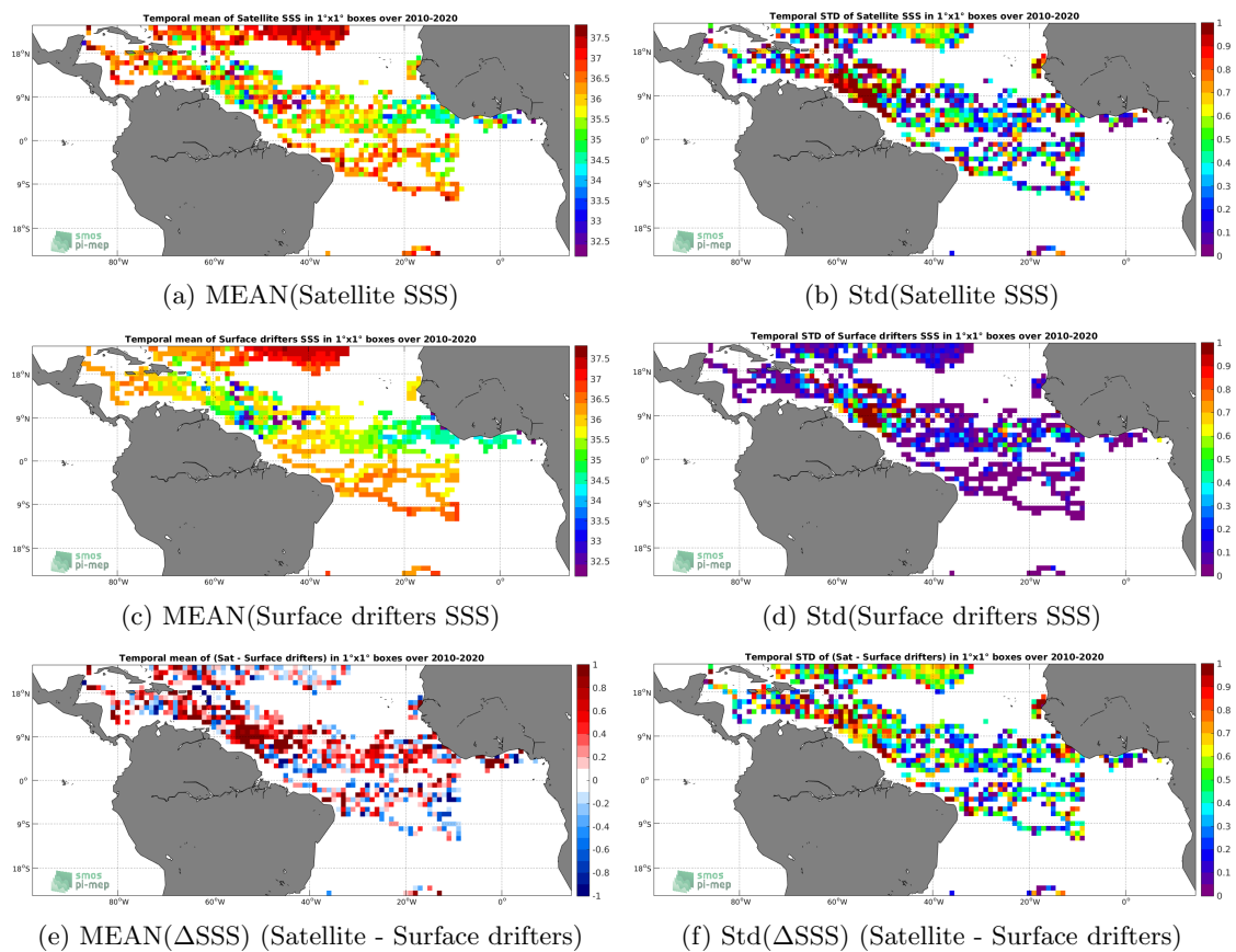
Figure 5: Temporal mean (left) and Std (right) of SSS from SMOS SSS L2 v662 (ESA) (top), Surface drifters (middle), and of \Delta SSS (Satellite - Surface drifters). Only match-up pairs are used to generate these maps.
