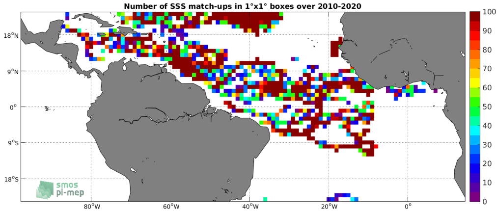
Figure 3: Number of SSS match-ups between Surface drifters SSS and the SMOS SSS L2 v662 (ESA) SSS product for the Tropical Atlantic Ocean Pi-MEP region over 1^\circ \times 1^\circ boxes and for the full satellite product period.
