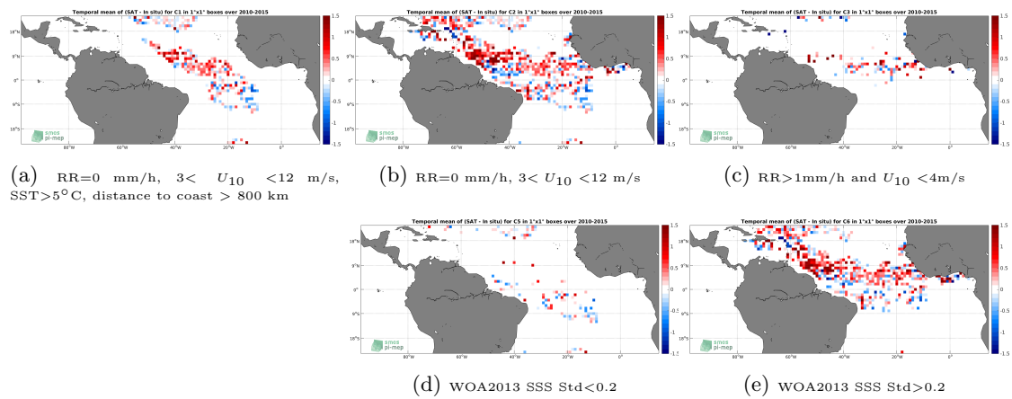
Figure 11: Temporal mean gridded over spatial boxes of size 1^\circ \times 1^\circ of \Delta\text{SSS} (SMOS SSS L2 v662 (ESA) - Surface drifters) for 5 different subdatasets corresponding to:RR=0 mm/h, 3 < U_{10} < 12 m/s, SST >5^\circ\text{C} , distance to coast > 800 km (a), RR=0 mm/h, 3 < U_{10} < 12 m/s (b), RR >1 mm/h and U_{10} < 4 m/s (c), WOA2013 SSS Std <0.2 (d), WOA2013 SSS Std >0.2 (e).
