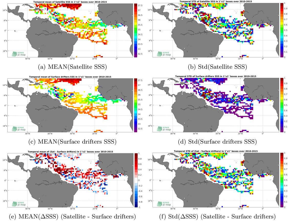
Figure 5: Temporal mean (left) and Std (right) of SSS from SMOS L2 v662 (ESA) (top), Surface drifters (middle), and of \Delta SSS (Satellite - Surface drifters). Only match-up pairs are used to generate these maps.
