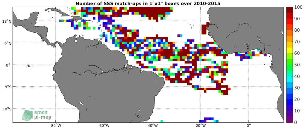
Figure 3: Number of SSS match-ups between Surface drifters SSS and the SMOS L2 v662 (ESA) SSS product for the Tropical Atlantic Ocean Pi-MEP region over 1^\circ \times 1^\circ boxes and for the full satellite product period.
