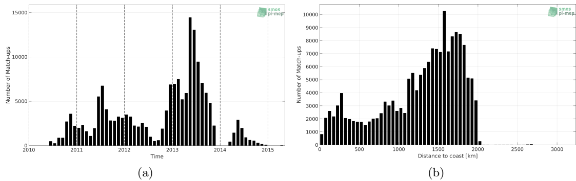
Figure 1: Number of match-ups between Surface drifters and SMOS L2 v662 (ESA) SSS as a function of time (a) and as function of the distance to coast (b) over the Tropical Atlantic Ocean Pi-MEP region and for the full satellite product period.
