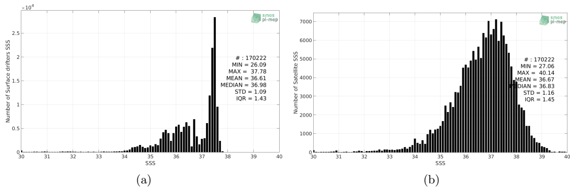
Figure 2: Histograms of SSS from Surface drifters (a) and SMOS L2 v662 (ESA) (b) considering all match-up pairs per bins of 0.1 over the Tropical Atlantic Ocean Pi-MEP region and for the full satellite product period.
