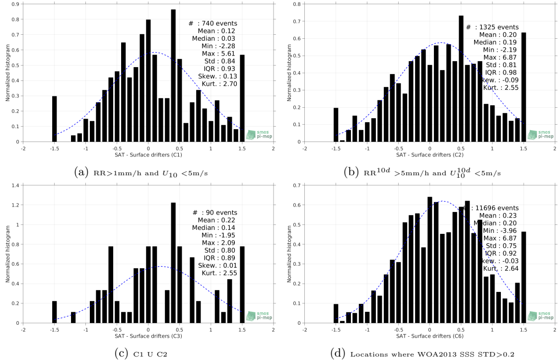
Figure 12: Normalized histogram of \Delta SSS (SMOS-L2-DPGS-v662 - Surface drifters) for 6 different subdatasets corresponding to: RR > 1mm/h and U_{10} < 5 m/s (a), RR^{10d} > 5 mm/h and U_{10}^{10d} < 5 m/s (b), C1 U C2 (c), Locations where WOA2013 SSS STD > 0.2 (d).
