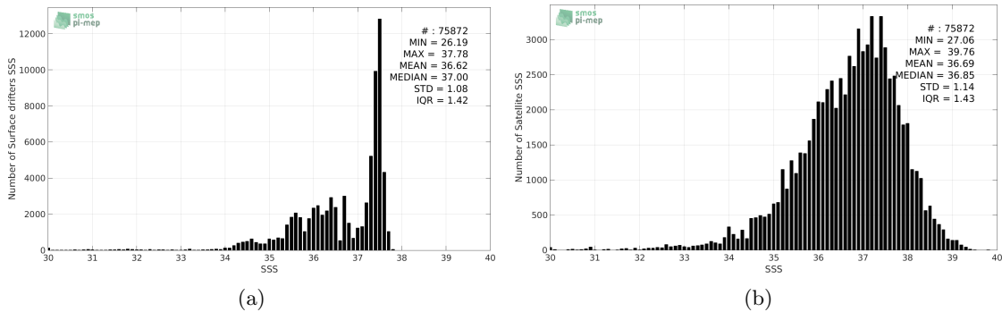
Figure 2: Histograms of SSS from Surface drifters (a) and SMOS-L2-DPGS-v662 (b) considering all match-up pairs per bins of 0.1 over the Tropical Atlantic Ocean Pi-MEP region and for the full satellite product period.
