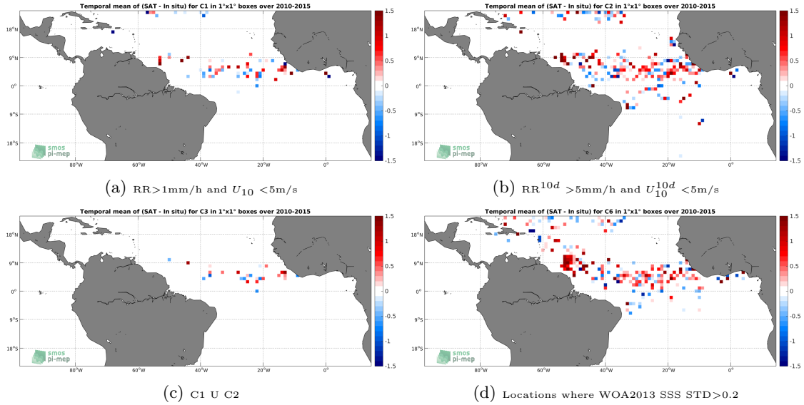
Figure 11: Temporal mean gridded over spatial boxes of size 1^\circ \times 1^\circ of \Delta SSS (SMOS-L2-DPGS-v662 - Surface drifters) for 4 different subdatasets corresponding to: RR > 1\text{mm/h} and U_{10} < 5\text{m/s} (a), RR^{10d} > 5\text{mm/h} and U_{10}^{10d} < 5\text{m/s} (b), C1 U C2 (c), Locations where WOA2013 SSS STD > 0.2 (d).
