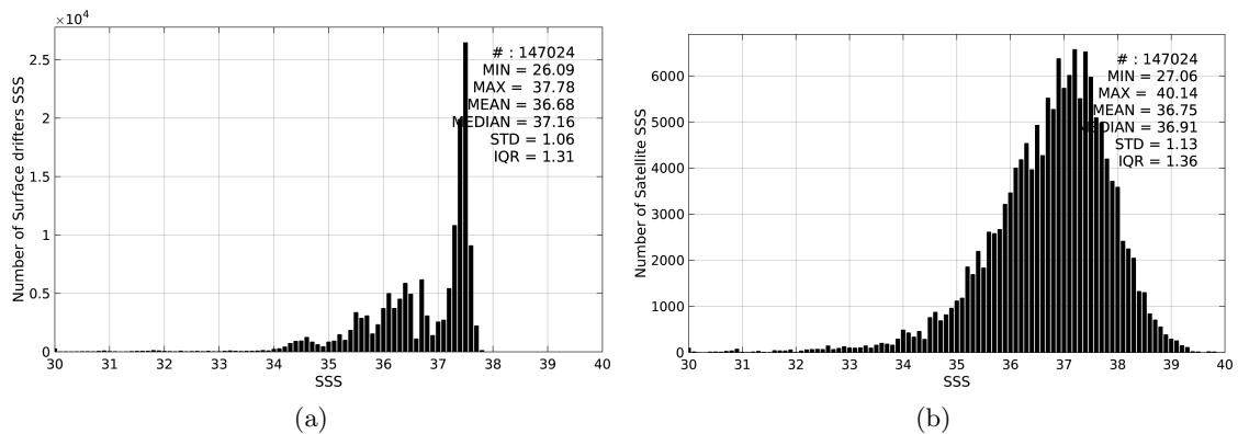
Figure 2: Histograms of SSS from Surface drifters (a) and SMOS-L2-DPGS-v662 (b) considering all match-up pairs per bins of 0.1 over the Tropical Atlantic Ocean Pi-MEP region and for the full satellite product period.
