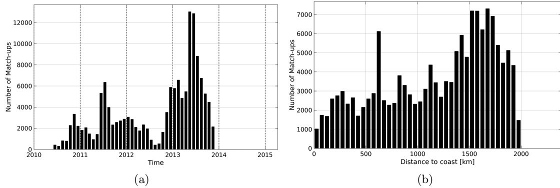
Figure 1: Number of match-ups between Surface drifters and SMOS-L2-DPGS-v662 SSS as a function of time (a) and as function of the distance to coast (b) over the Tropical Atlantic Ocean Pi-MEP region and for the full satellite product period.
