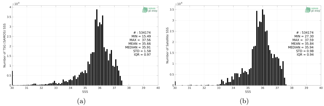
Figure 2: Histograms of SSS from TSG (SAMOS) (a) and SMAP SSS L4 OI v1 - 7 Days (IPRC) (b) considering all match-up pairs per bins of 0.1 over the Tropical Atlantic Ocean Pi-MEP region and for the full satellite product period.
