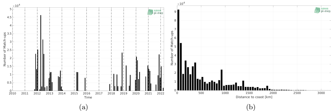
Figure 1: Number of match-ups between TSG (SAMOS) and SMAP SSS L4 OI v1 - 7 Days (IPRC) SSS as a function of time (a) and as function of the distance to coast (b) over the Tropical Atlantic Ocean Pi-MEP region and for the full satellite product period.
