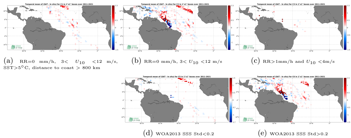
Figure 12: Temporal mean gridded over spatial boxes of size 1^\circ \times 1^\circ of \Delta\text{SSS} (SMAP SSS L4 OI v1 - 7 Days (IPRC) - TSG (SAMOS)) for 5 different subdatasets corresponding to:RR=0 mm/h, 3 < U_{10} < 12 m/s, SST >5^\circ\text{C} , distance to coast > 800 km (a), RR=0 mm/h, 3 < U_{10} < 12 m/s (b), RR >1 mm/h and U_{10} < 4 m/s (c), WOA2013 SSS Std <0.2 (d), WOA2013 SSS Std >0.2 (e).
