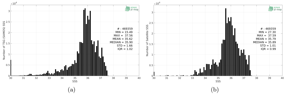
Figure 2: Histograms of SSS from TSG (SAMOS) (a) and SMAP SSS L4 OI v1 - 7day (IPRC) (b) considering all match-up pairs per bins of 0.1 over the Tropical Atlantic Ocean Pi-MEP region and for the full satellite product period.
