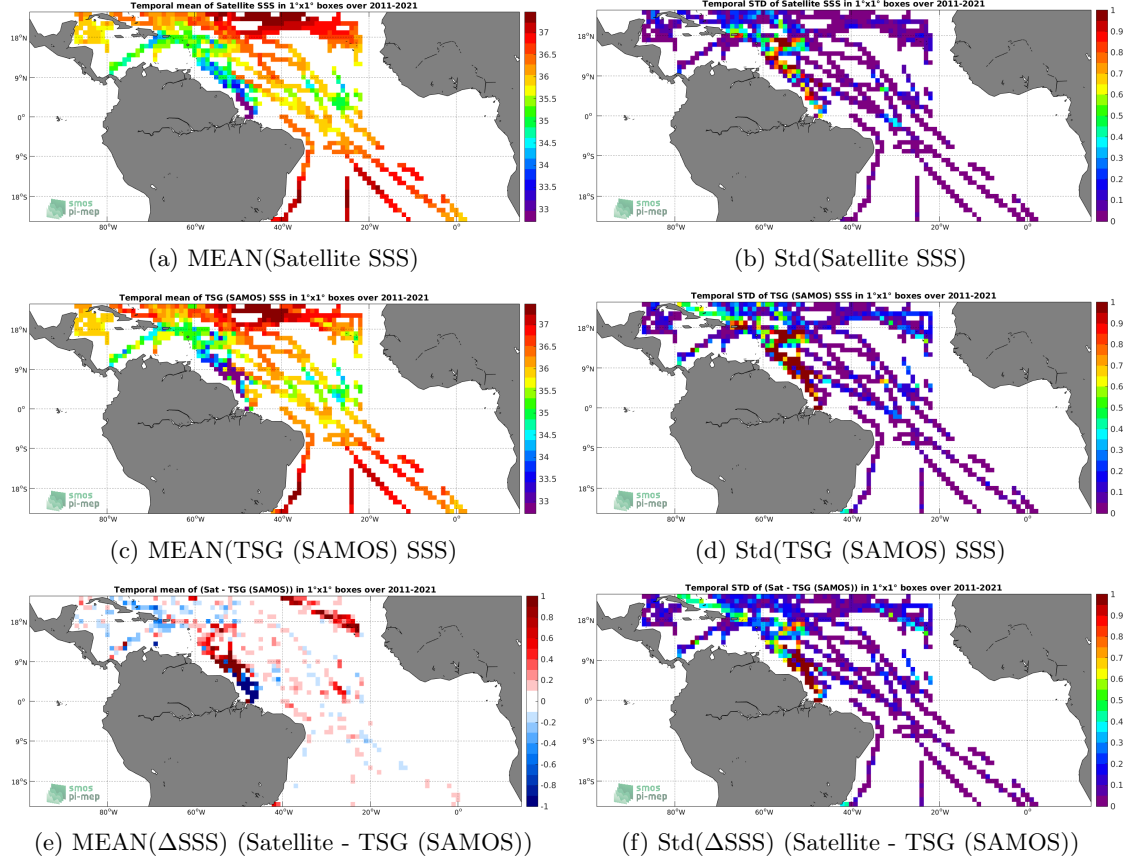
Figure 6: Temporal mean (left) and Std (right) of SSS from SMAP SSS L4 OI v1 - 7day (IPRC) (top), TSG (SAMOS) (middle), and of \Delta SSS (Satellite - TSG (SAMOS)). Only match-up pairs are used to generate these maps.
