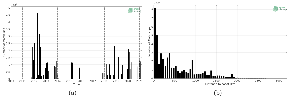
Figure 1: Number of match-ups between TSG (SAMOS) and SMAP SSS L4 OI v1 - 7day (IPRC) SSS as a function of time (a) and as function of the distance to coast (b) over the Tropical Atlantic Ocean Pi-MEP region and for the full satellite product period.
