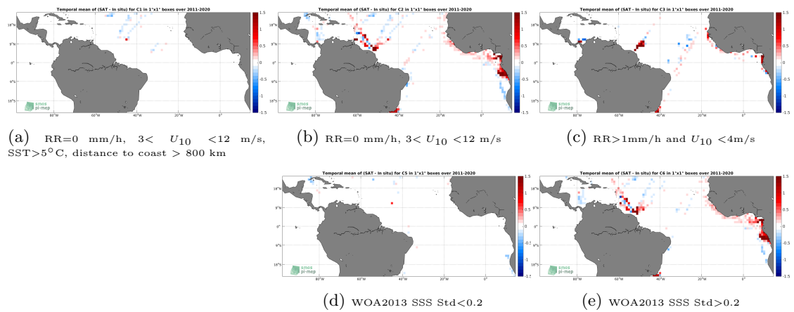
Figure 12: Temporal mean gridded over spatial boxes of size 1^\circ \times 1^\circ of \Delta SSS (SMAP SSS L4 OI v1 - 7 Days (IPRC) - TSG (LEGOS-DM)) for 5 different subdatasets corresponding to: RR=0 mm/h, 3 < U_{10} < 12 m/s, SST > 5°C, distance to coast > 800 km (a), RR=0 mm/h, 3 < U_{10} < 12 m/s (b), RR > 1mm/h and U_{10} < 4 m/s (c), WOA2013 SSS Std < 0.2 (d), WOA2013 SSS Std > 0.2 (e).
