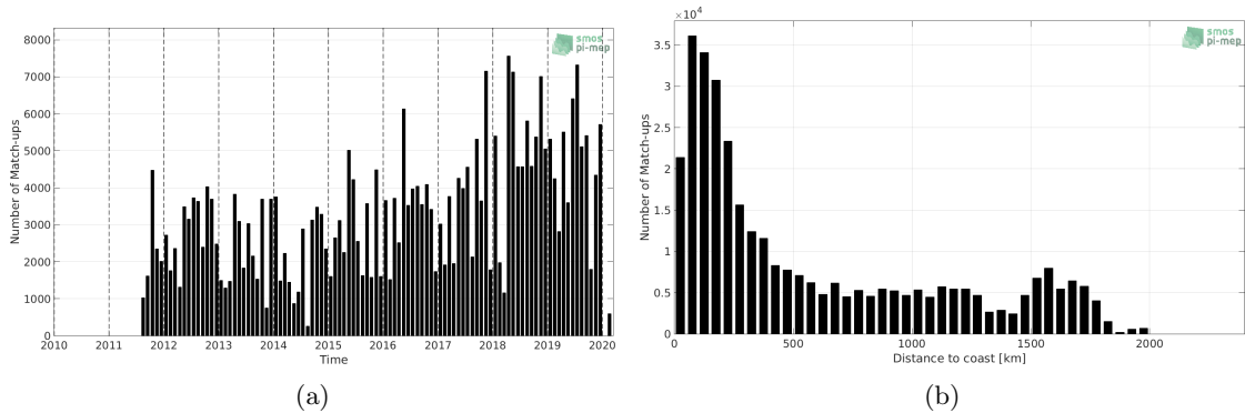
Figure 1: Number of match-ups between TSG (LEGOS-DM) and SMAP SSS L4 OI v1 - 7day (IPRC) SSS as a function of time (a) and as function of the distance to coast (b) over the Tropical Atlantic Ocean Pi-MEP region and for the full satellite product period.
