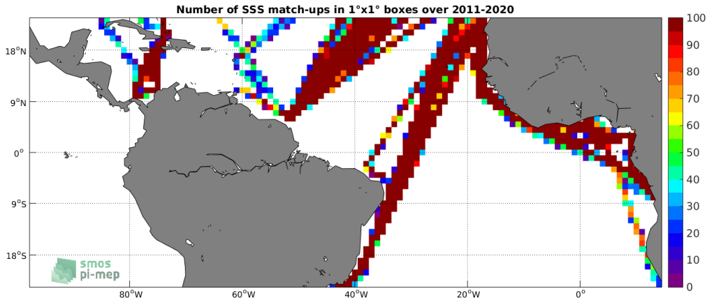
Figure 4: Number of SSS match-ups between TSG (LEGOS-DM) SSS and the SMAP SSS L4 OI v1 - 7day (IPRC) SSS product for the Tropical Atlantic Ocean Pi-MEP region over 1^\circ \times 1^\circ boxes and for the full satellite product period.
