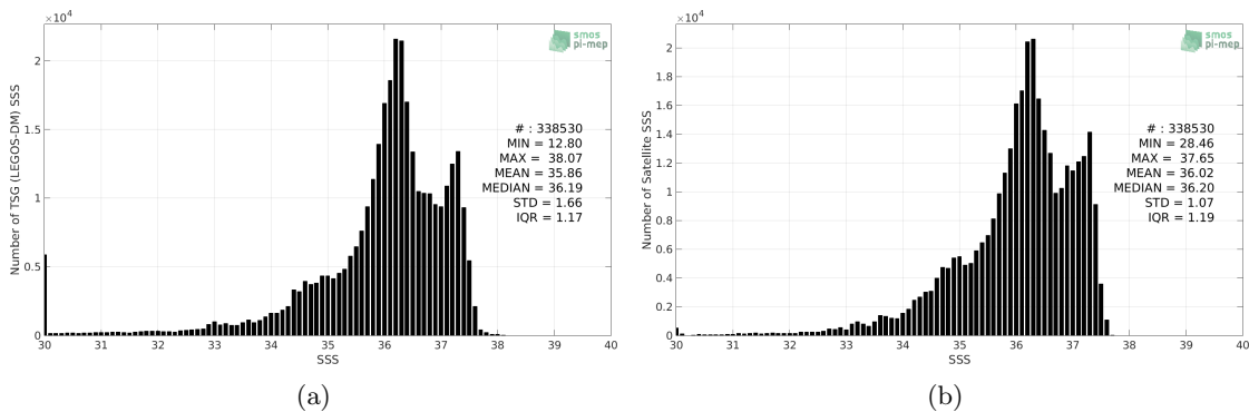
Figure 2: Histograms of SSS from TSG (LEGOS-DM) (a) and SMAP SSS L4 OI v1 - 7day (IPRC) (b) considering all match-up pairs per bins of 0.1 over the Tropical Atlantic Ocean Pi-MEP region and for the full satellite product period.
