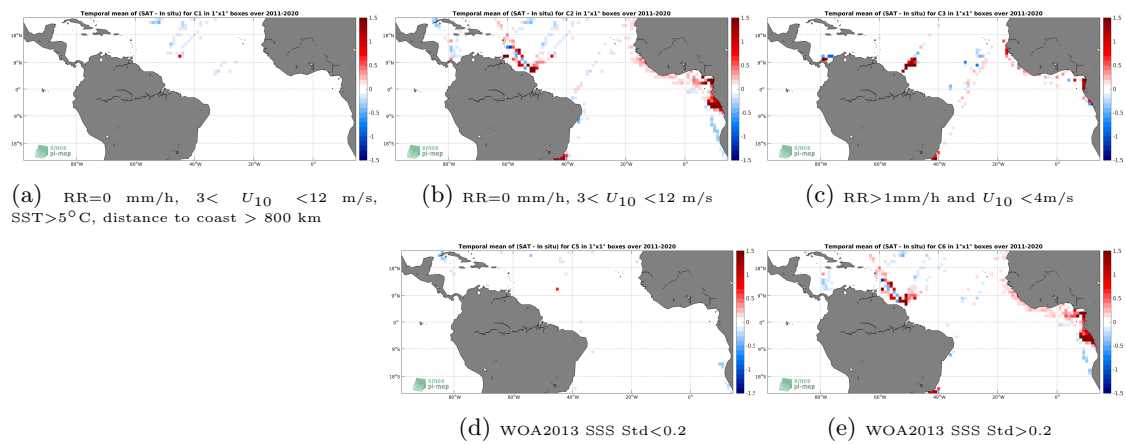
Figure 12: Temporal mean gridded over spatial boxes of size 1^\circ \times 1^\circ of \Delta SSS (SMAP SSS L4 OI v1 - 7day (IPRC) - TSG (LEGOS-DM)) for 5 different subdatasets corresponding to:RR=0 mm/h, 3 < U_{10} < 12 m/s, SST>5°C, distance to coast > 800 km (a), RR=0 mm/h, 3 < U_{10} < 12 m/s (b), RR>1mm/h and U_{10} < 4 m/s (c), WOA2013 SSS Std<0.2 (d), WOA2013 SSS Std>0.2 (e).
