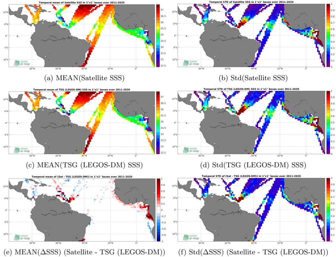
Figure 6: Temporal mean (left) and Std (right) of SSS from SMAP SSS L4 OI v1 - 7day (IPRC) (top), TSG (LEGOS-DM) (middle), and of \Delta SSS (Satellite - TSG (LEGOS-DM)). Only match-up pairs are used to generate these maps.
