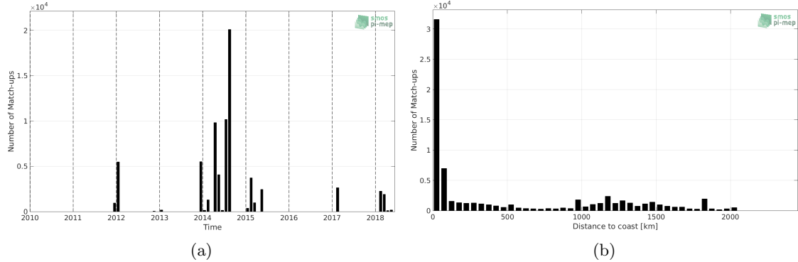
Figure 1: Number of match-ups between TSG (GOSUD-Sailing-ship) and SMAP SSS L4 OI v1 - 7 Days (IPRC) SSS as a function of time (a) and as function of the distance to coast (b) over the Tropical Atlantic Ocean Pi-MEP region and for the full satellite product period.
