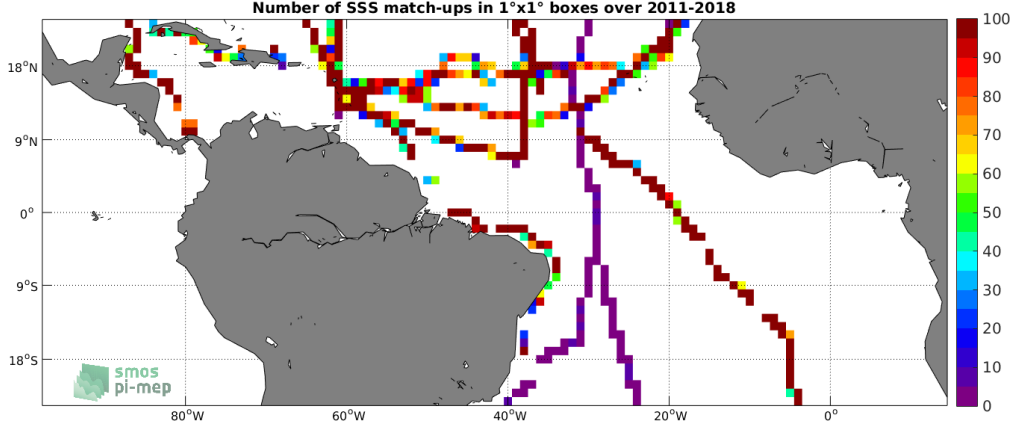
Figure 4: Number of SSS match-ups between TSG (GOSUD-Sailing-ship) SSS and the SMAP SSS L4 OI v1 - 7 Days (IPRC) SSS product for the Tropical Atlantic Ocean Pi-MEP region over 1^\circ \times 1^\circ boxes and for the full satellite product period.
