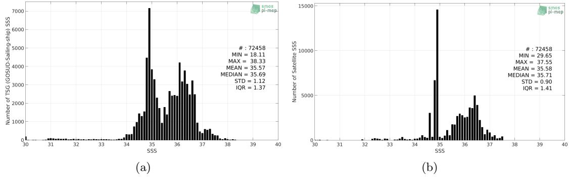
Figure 2: Histograms of SSS from TSG (GOSUD-Sailing-ship) (a) and SMAP SSS L4 OI v1 - 7 Days (IPRC) (b) considering all match-up pairs per bins of 0.1 over the Tropical Atlantic Ocean Pi-MEP region and for the full satellite product period.
