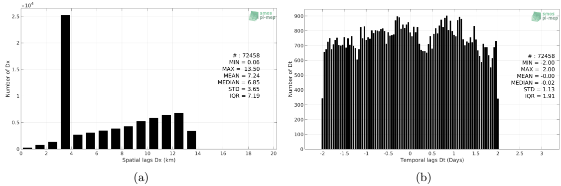
Figure 5: Histograms of the spatial (a) and temporal (b) lags between the location/time of the TSG (GOSUD-Sailing-ship) measurement and the date of the corresponding SMAP SSS L4 OI v1 - 7day (IPRC) SSS pixel.
