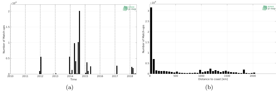
Figure 1: Number of match-ups between TSG (GOSUD-Sailing-ship) and SMAP SSS L4 OI v1 - 7day (IPRC) SSS as a function of time (a) and as function of the distance to coast (b) over the Tropical Atlantic Ocean Pi-MEP region and for the full satellite product period.
