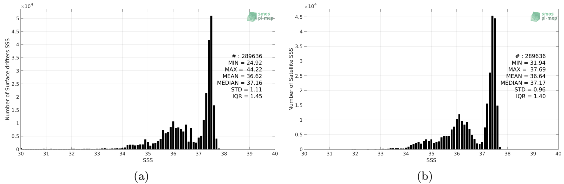
Figure 2: Histograms of SSS from Surface drifters (a) and SMAP SSS L4 OI v1 - 7 Days (IPRC) (b) considering all match-up pairs per bins of 0.1 over the Tropical Atlantic Ocean Pi-MEP region and for the full satellite product period.
