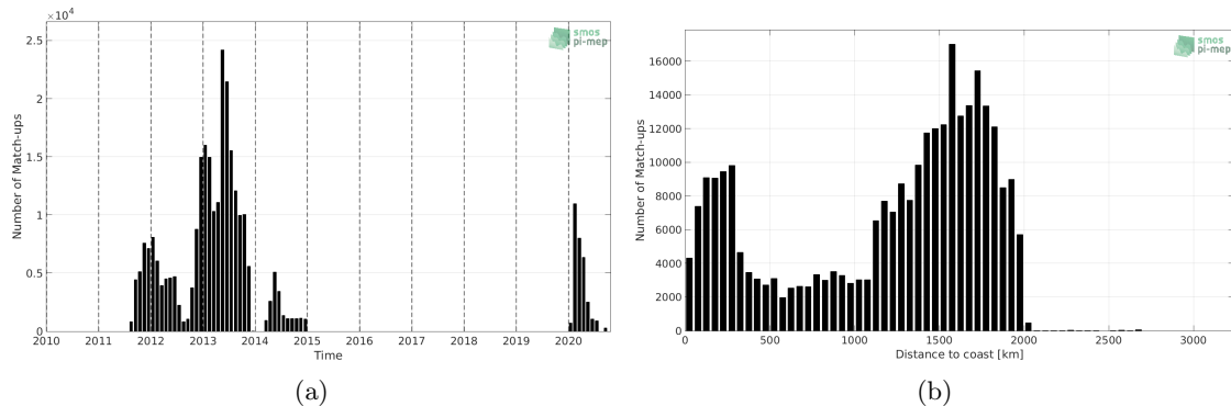
Figure 1: Number of match-ups between Surface drifters and SMAP SSS L4 OI v1 - 7 Days (IPRC) SSS as a function of time (a) and as function of the distance to coast (b) over the Tropical Atlantic Ocean Pi-MEP region and for the full satellite product period.
