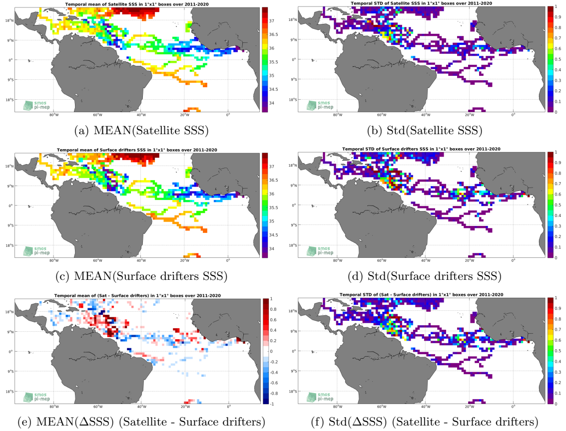
Figure 5: Temporal mean (left) and Std (right) of SSS from SMAP SSS L4 OI v1 - 7 Days (IPRC) (top), Surface drifters (middle), and of \Delta SSS (Satellite - Surface drifters). Only match-up pairs are used to generate these maps.
