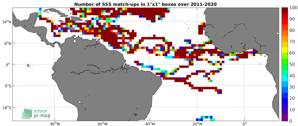
Figure 3: Number of SSS match-ups between Surface drifters SSS and the SMAP SSS L4 OI v1 - 7 Days (IPRC) SSS product for the Tropical Atlantic Ocean Pi-MEP region over 1^\circ \times 1^\circ boxes and for the full satellite product period.
