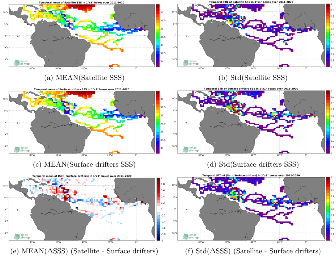
Figure 5: Temporal mean (left) and Std (right) of SSS from SMAP SSS L4 OI v1 - 7day (IPRC) (top), Surface drifters (middle), and of \Delta SSS (Satellite - Surface drifters). Only match-up pairs are used to generate these maps.
