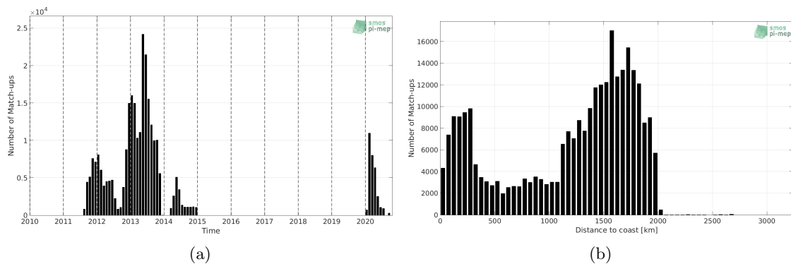
Figure 1: Number of match-ups between Surface drifters and SMAP SSS L4 OI v1 - 7day (IPRC) SSS as a function of time (a) and as function of the distance to coast (b) over the Tropical Atlantic Ocean Pi-MEP region and for the full satellite product period.
