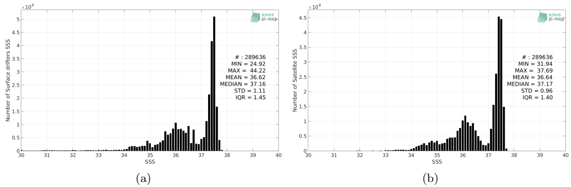
Figure 2: Histograms of SSS from Surface drifters (a) and SMAP SSS L4 OI v1 - 7day (IPRC) (b) considering all match-up pairs per bins of 0.1 over the Tropical Atlantic Ocean Pi-MEP region and for the full satellite product period.
