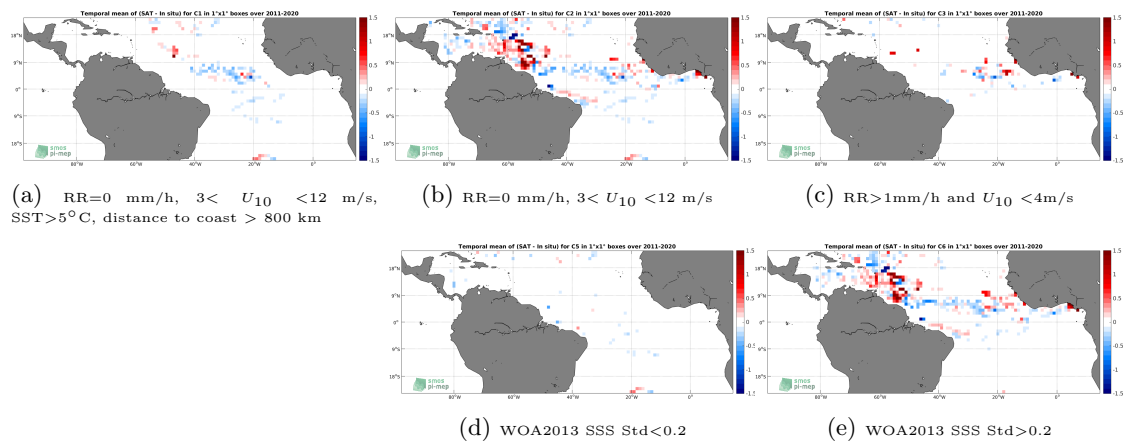
Figure 11: Temporal mean gridded over spatial boxes of size 1^\circ \times 1^\circ of \Delta SSS (SMAP SSS L4 OI v1 - 7day (IPRC) - Surface drifters) for 5 different subdatasets corresponding to:RR=0 mm/h, 3 < U_{10} < 12 m/s, SST>5°C, distance to coast > 800 km (a), RR=0 mm/h, 3 < U_{10} < 12 m/s (b), RR>1mm/h and U_{10} < 4 m/s (c), WOA2013 SSS Std<0.2 (d), WOA2013 SSS Std>0.2 (e).
