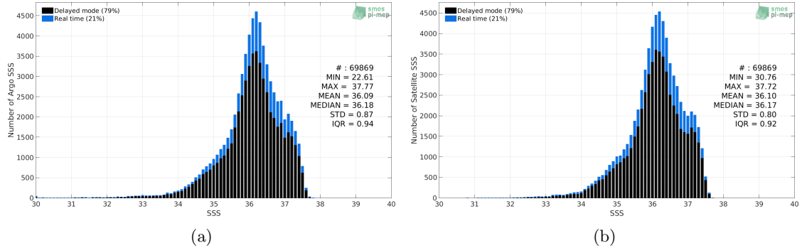
Figure 2: Histograms of SSS from Argo (a) and SMAP SSS L4 OI v1 - 7 Days (IPRC) (b) considering all match-up pairs per bins of 0.1 over the Tropical Atlantic Ocean Pi-MEP region and for the full satellite product period.
