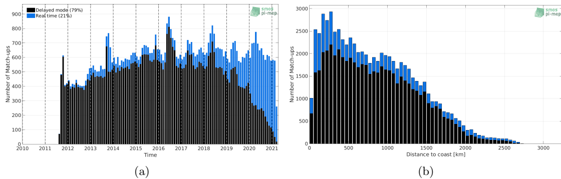
Figure 1: Number of match-ups between Argo and SMAP SSS L4 OI v1 - 7 Days (IPRC) SSS as a function of time (a) and as function of the distance to coast (b) over the Tropical Atlantic Ocean Pi-MEP region and for the full satellite product period.
