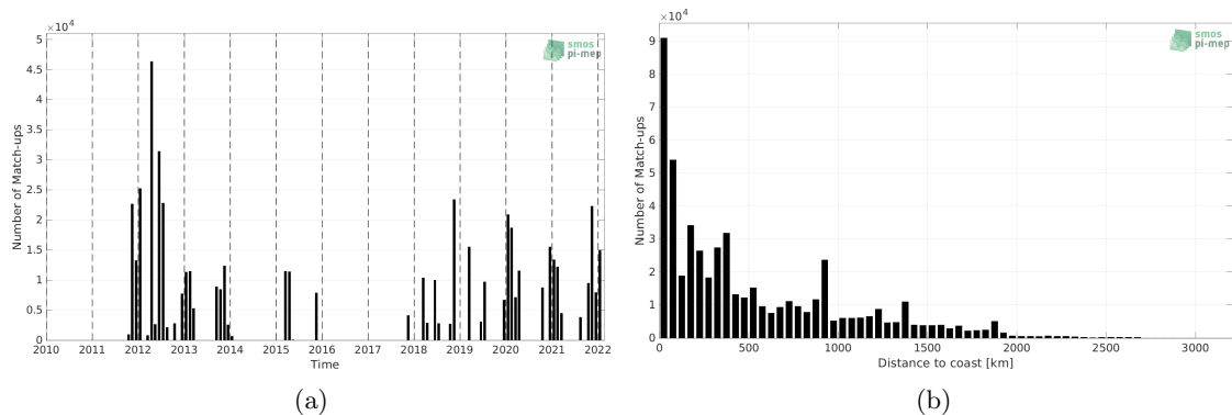
Figure 1: Number of match-ups between TSG (SAMOS) and SMAP SSS L4 OI v1 - Monthly (IPRC) SSS as a function of time (a) and as function of the distance to coast (b) over the Tropical Atlantic Ocean Pi-MEP region and for the full satellite product period.
