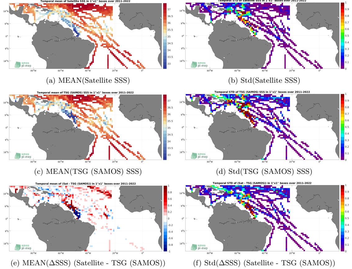
Figure 6: Temporal mean (left) and Std (right) of SSS from SMAP SSS L4 OI v1 - Monthly (IPRC) (top), TSG (SAMOS) (middle), and of \Delta\text{SSS}(\text{Satellite} - \text{TSG}(\text{SAMOS})) . Only match-up pairs are used to generate these maps.
