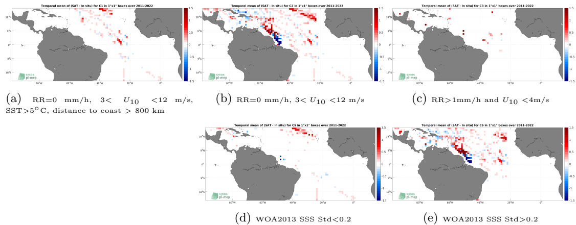
Figure 12: Temporal mean gridded over spatial boxes of size 1^\circ \times 1^\circ of \Delta SSS (SMAP SSS L4 OI v1 - Monthly (IPRC) - TSG (SAMOS)) for 5 different subdatasets corresponding to:RR=0 mm/h, 3 < U_{10} < 12 m/s, SST >5^\circ\text{C} , distance to coast > 800 km (a), RR=0 mm/h, 3 < U_{10} < 12 m/s (b), RR >1 mm/h and U_{10} < 4 m/s (c), WOA2013 SSS Std <0.2 (d), WOA2013 SSS Std >0.2 (e).
