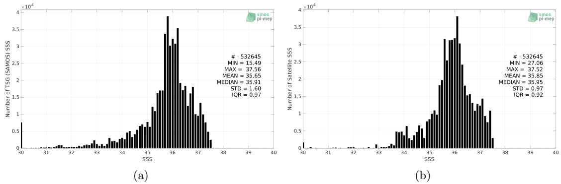
Figure 2: Histograms of SSS from TSG (SAMOS) (a) and SMAP SSS L4 OI v1 - Monthly (IPRC) (b) considering all match-up pairs per bins of 0.1 over the Tropical Atlantic Ocean Pi-MEP region and for the full satellite product period.
