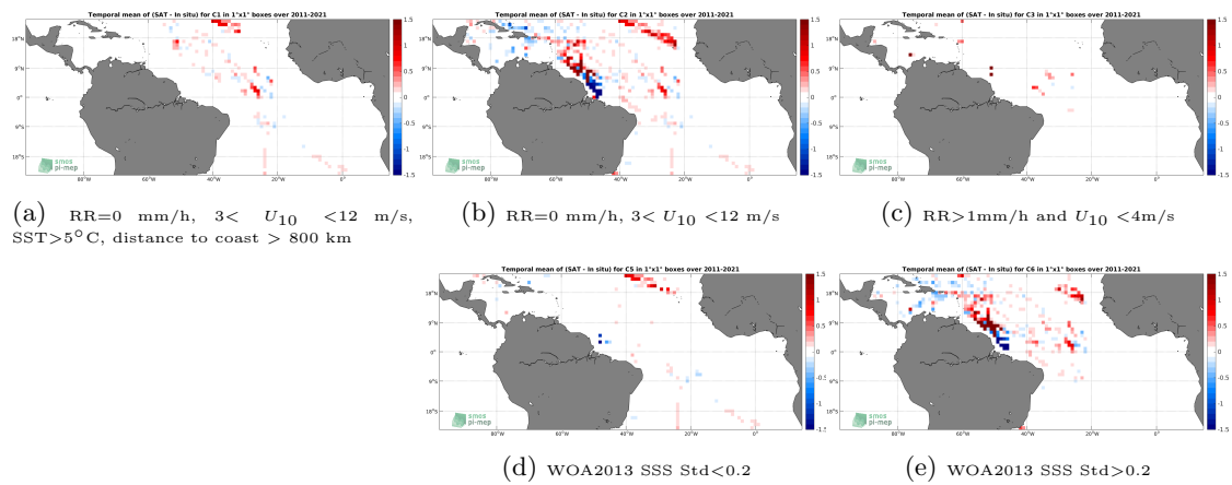
Figure 12: Temporal mean gridded over spatial boxes of size 1^\circ \times 1^\circ of \Delta\text{SSS} (SMAP SSS L4 OI v1 - Monthly (IPRC) - TSG (SAMOS)) for 5 different subdatasets corresponding to:RR=0 mm/h, 3 < U_{10} < 12 m/s, SST >5^\circ\text{C} , distance to coast > 800 km (a), RR=0 mm/h, 3 < U_{10} < 12 m/s (b), RR >1 mm/h and U_{10} < 4 m/s (c), WOA2013 SSS Std <0.2 (d), WOA2013 SSS Std >0.2 (e).
