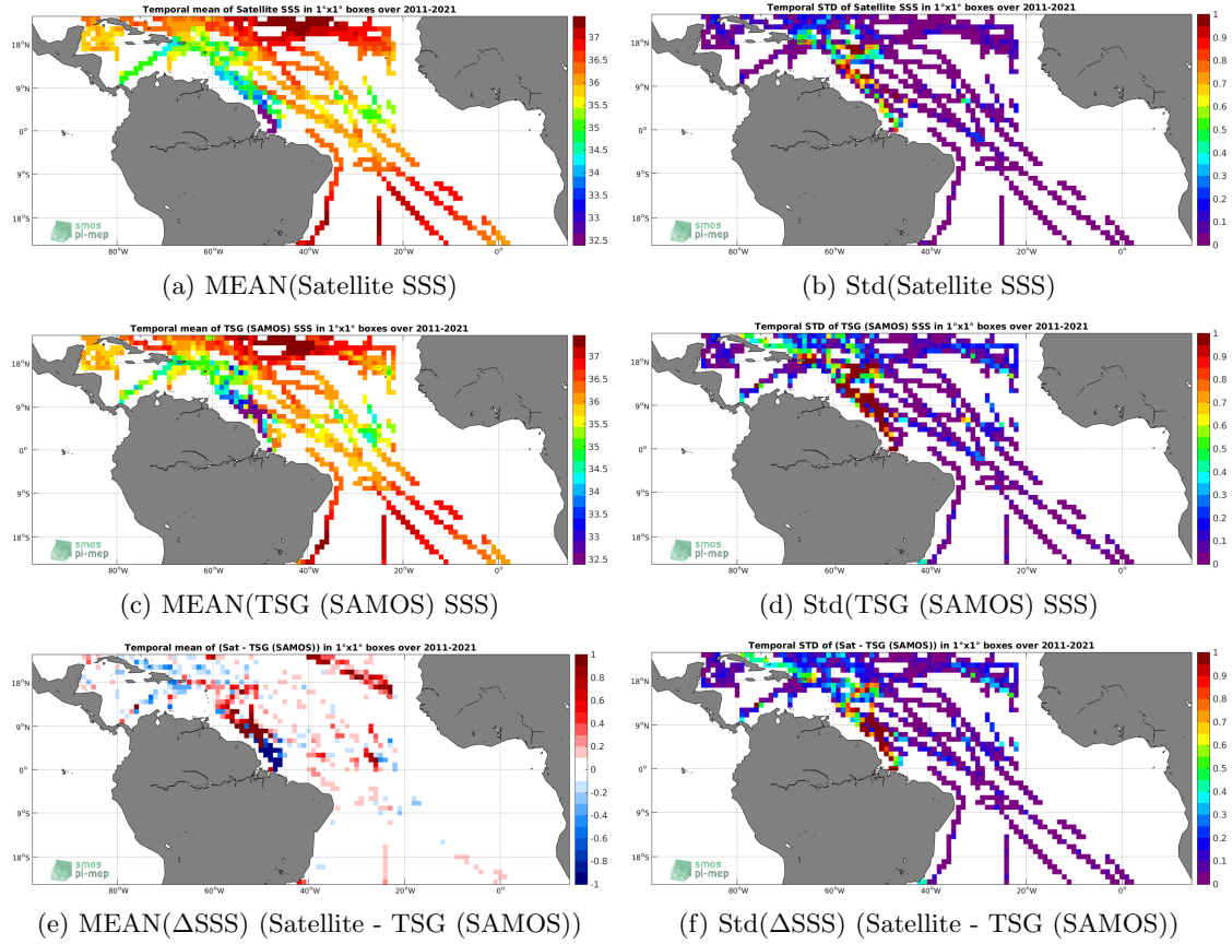
Figure 6: Temporal mean (left) and Std (right) of SSS from SMAP SSS L4 OI v1 - Monthly (IPRC) (top), TSG (SAMOS) (middle), and of \Delta SSS (Satellite - TSG (SAMOS)). Only match-up pairs are used to generate these maps.
