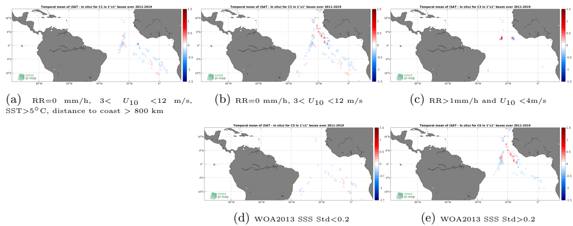
Figure 12: Temporal mean gridded over spatial boxes of size 1^\circ \times 1^\circ of \Delta SSS (SMAP SSS L4 OI v1 - Monthly (IPRC) - TSG (Polarstern)) for 5 different subdatasets corresponding to: RR=0 mm/h, 3 < U_{10} < 12 m/s, SST > 5°C, distance to coast > 800 km (a), RR=0 mm/h, 3 < U_{10} < 12 m/s (b), RR > 1mm/h and U_{10} < 4 m/s (c), WOA2013 SSS Std < 0.2 (d), WOA2013 SSS Std > 0.2 (e).
