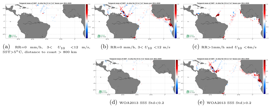
Figure 12: Temporal mean gridded over spatial boxes of size 1^\circ \times 1^\circ of \Delta\text{SSS} (SMAP SSS L4 OI v1 - Monthly (IPRC) - TSG (LEGOS-DM)) for 5 different subdatasets corresponding to:RR=0 mm/h, 3 < U_{10} < 12 m/s, SST >5^\circ\text{C} , distance to coast > 800 km (a), RR=0 mm/h, 3 < U_{10} < 12 m/s (b), RR >1 mm/h and U_{10} < 4 m/s (c), WOA2013 SSS Std <0.2 (d), WOA2013 SSS Std >0.2 (e).
