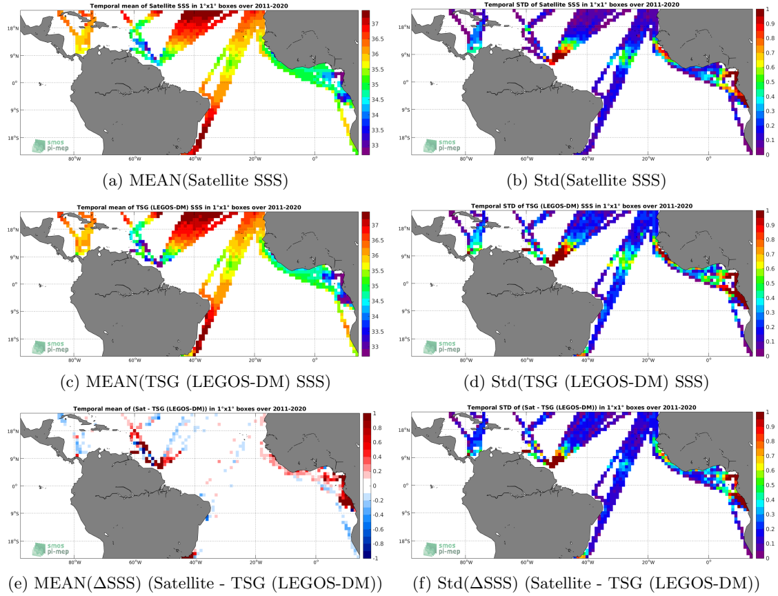
Figure 6: Temporal mean (left) and Std (right) of SSS from SMAP SSS L4 OI v1 - Monthly (IPRC) (top), TSG (LEGOS-DM) (middle), and of \Delta\text{SSS} (Satellite - TSG (LEGOS-DM)). Only match-up pairs are used to generate these maps.
