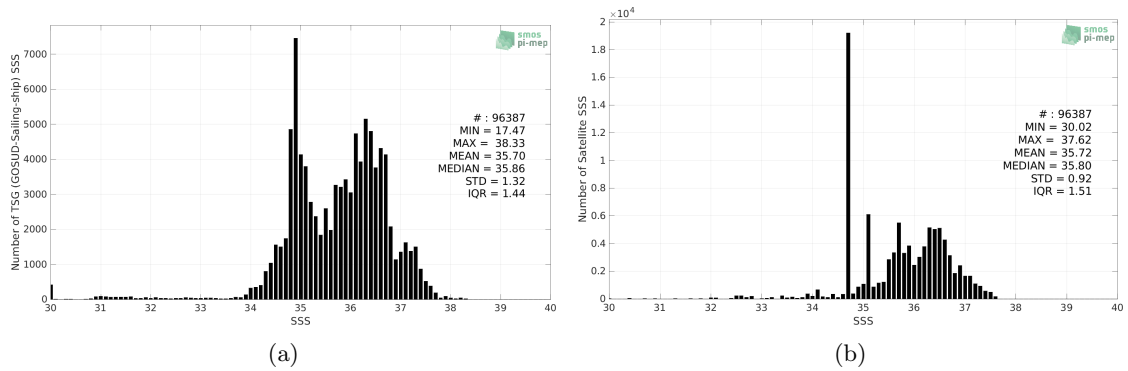
Figure 2: Histograms of SSS from TSG (GOSUD-Sailing-ship) (a) and SMAP SSS L4 OI v1 - Monthly (IPRC) (b) considering all match-up pairs per bins of 0.1 over the Tropical Atlantic Ocean Pi-MEP region and for the full satellite product period.
