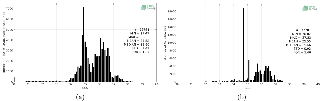
Figure 2: Histograms of SSS from TSG (GOSUD-Sailing-ship) (a) and SMAP SSS L4 OI v1 - Monthly (IPRC) (b) considering all match-up pairs per bins of 0.1 over the Tropical Atlantic Ocean Pi-MEP region and for the full satellite product period.
