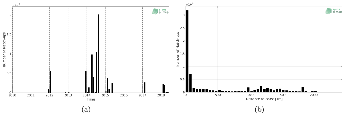
Figure 1: Number of match-ups between TSG (GOSUD-Sailing-ship) and SMAP SSS L4 OI v1 - Monthly (IPRC) SSS as a function of time (a) and as function of the distance to coast (b) over the Tropical Atlantic Ocean Pi-MEP region and for the full satellite product period.
