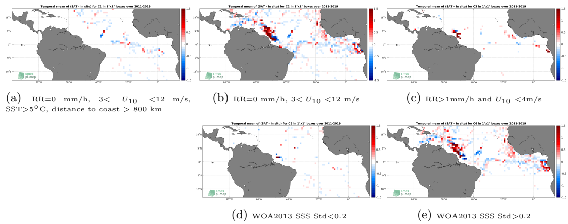
Figure 12: Temporal mean gridded over spatial boxes of size 1^\circ \times 1^\circ of \Delta\text{SSS} (SMAP SSS L4 OI v1 - Monthly (IPRC) - TSG (GOSUD-Research-vessel)) for 5 different subdatasets corresponding to:RR=0 mm/h, 3 < U_{10} < 12 m/s, SST>5°C, distance to coast > 800 km (a), RR=0 mm/h, 3 < U_{10} < 12 m/s (b), RR>1mm/h and U_{10} < 4 m/s (c), WOA2013 SSS Std<0.2 (d), WOA2013 SSS Std>0.2 (e).
