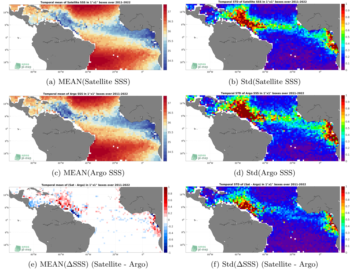
Figure 6: Temporal mean (left) and Std (right) of SSS from SMAP SSS L4 OI v1 - Monthly (IPRC) (top), Argo (middle), and of \Delta\text{SSS} (Satellite - Argo). Only match-up pairs are used to generate these maps.
