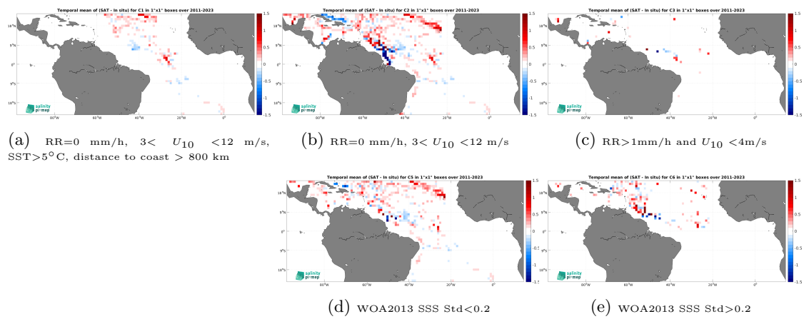
Figure 14: Temporal mean gridded over spatial boxes of size 1^\circ \times 1^\circ of \Delta\text{SSS} (SMAP SSS L4 OI v3 - Monthly (ESR) - TSG (SAMOS)) for 5 different subdatasets corresponding to:RR=0 mm/h, 3 < U_{10} < 12 m/s, SST >5^\circ\text{C} , distance to coast > 800 km (a), RR=0 mm/h, 3 < U_{10} < 12 m/s (b), RR >1 mm/h and U_{10} < 4 m/s (c), WOA2013 SSS Std <0.2 (d), WOA2013 SSS Std >0.2 (e).
