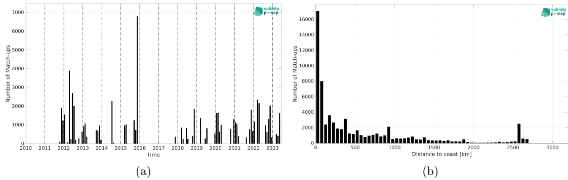
Figure 2: Number of match-ups between TSG (SAMOS) and SMAP SSS L4 OI v3 - Monthly (ESR) SSS as a function of time (a) and as function of the distance to coast (b) over the Tropical Atlantic Ocean Pi-MEP region and for the full satellite product period.
