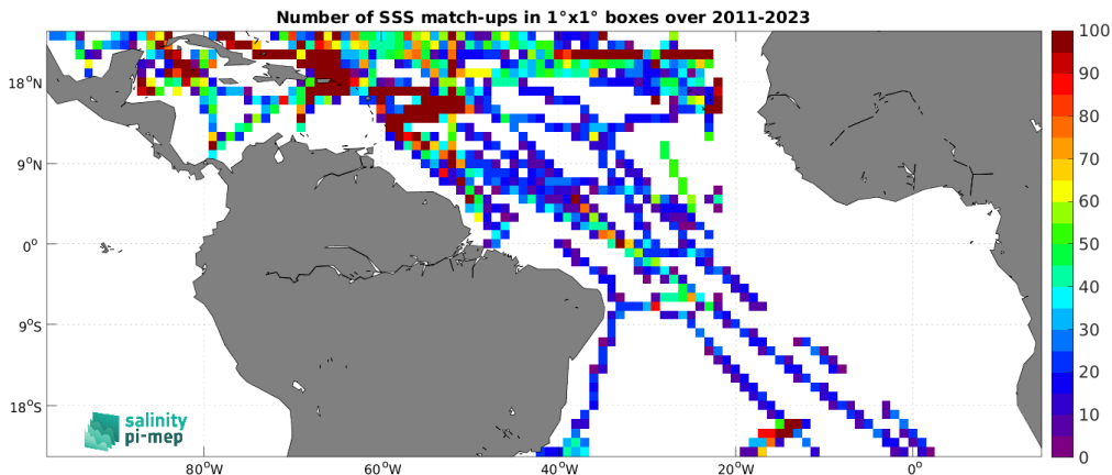
Figure 5: Number of SSS match-ups between TSG (SAMOS) SSS and the SMAP SSS L4 OI v3 - Monthly (ESR) SSS product for the Tropical Atlantic Ocean Pi-MEP region over 1^\circ \times 1^\circ boxes and for the full satellite product period.
