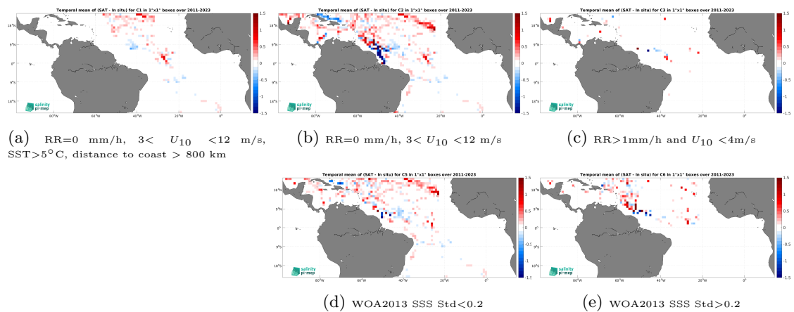
Figure 14: Temporal mean gridded over spatial boxes of size 1^\circ \times 1^\circ of \Delta\text{SSS} (SMAP SSS L4 OI v3 - Monthly (ESR) - TSG (SAMOS)) for 5 different subdatasets corresponding to:RR=0 mm/h, 3 < U_{10} < 12 m/s, SST >5^\circ\text{C} , distance to coast > 800 km (a), RR=0 mm/h, 3 < U_{10} < 12 m/s (b), RR >1 mm/h and U_{10} < 4 m/s (c), WOA2013 SSS Std <0.2 (d), WOA2013 SSS Std >0.2 (e).
