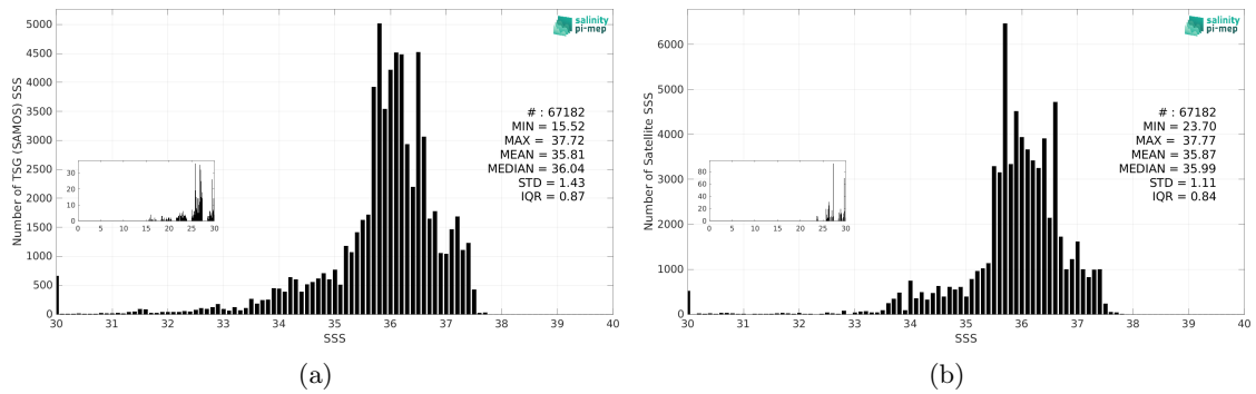
Figure 3: Histograms of SSS from TSG (SAMOS) (a) and SMAP SSS L4 OI v3 - Monthly (ESR) (b) considering all match-up pairs per bins of 0.1 over the Tropical Atlantic Ocean Pi-MEP region and for the full satellite product period.
