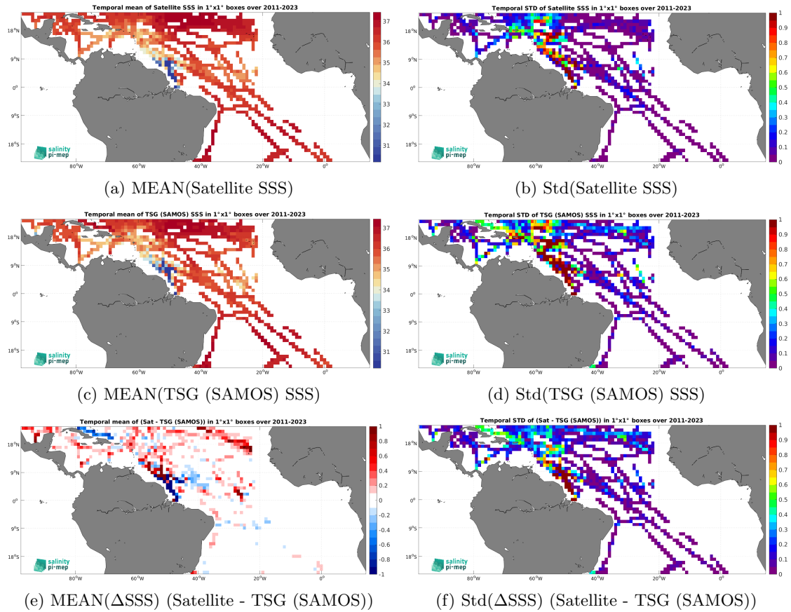
Figure 7: Temporal mean (left) and Std (right) of SSS from SMAP SSS L4 OI v3 - Monthly (ESR) (top), TSG (SAMOS) (middle), and of \Delta SSS (Satellite - TSG (SAMOS)). Only match-up pairs are used to generate these maps.
