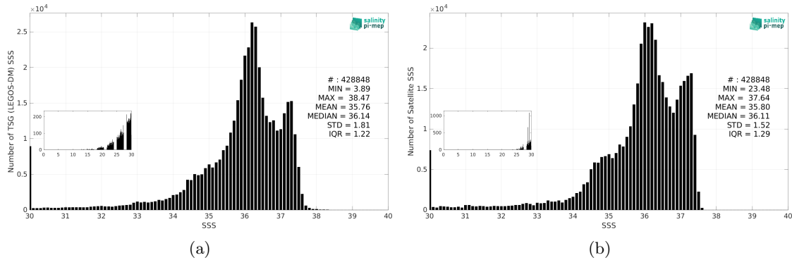
Figure 3: Histograms of SSS from TSG (LEGOS-DM) (a) and SMAP SSS L4 OI v3 - Monthly (ESR) (b) considering all match-up pairs per bins of 0.1 over the Tropical Atlantic Ocean Pi-MEP region and for the full satellite product period.
