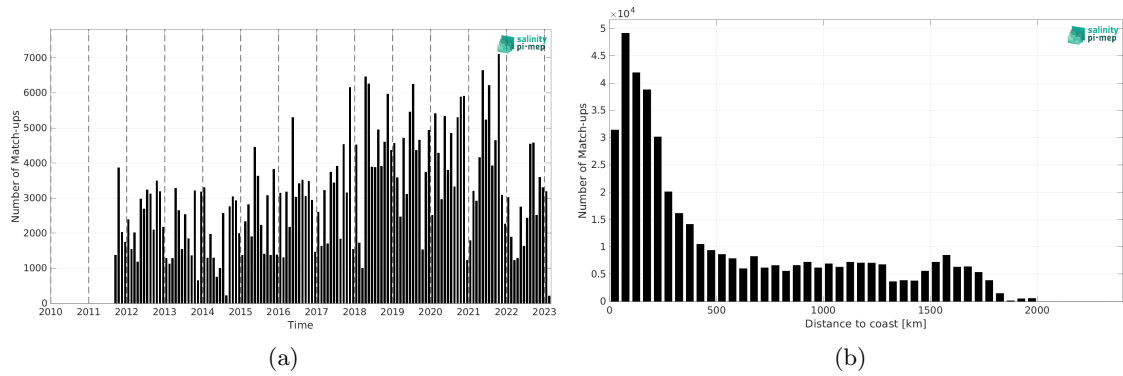
Figure 2: Number of match-ups between TSG (LEGOS-DM) and SMAP SSS L4 OI v3 - Monthly (ESR) SSS as a function of time (a) and as function of the distance to coast (b) over the Tropical Atlantic Ocean Pi-MEP region and for the full satellite product period.
