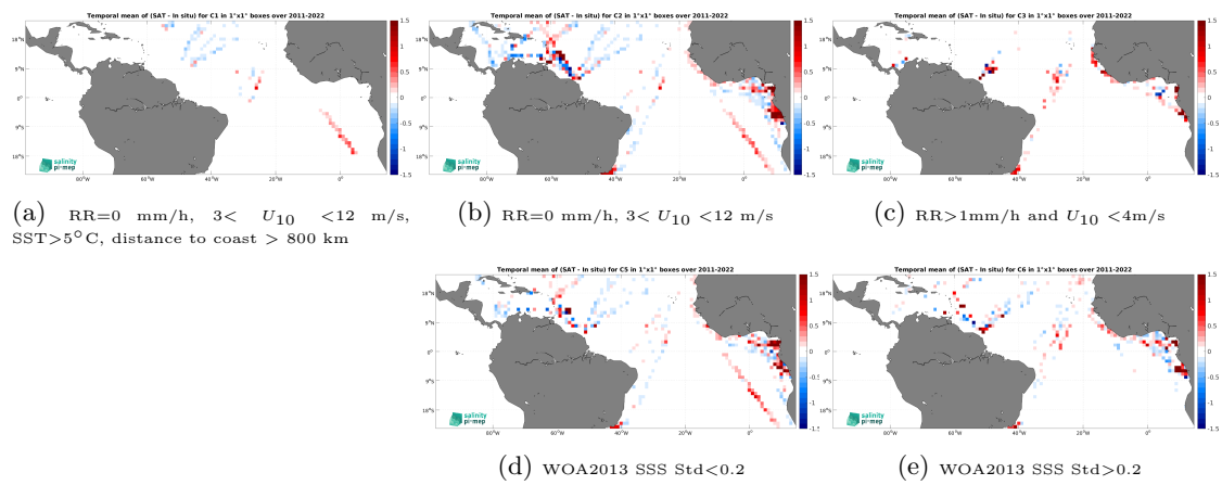
Figure 14: Temporal mean gridded over spatial boxes of size 1^\circ \times 1^\circ of \Delta\text{SSS} (SMAP SSS L4 OI v3 - Monthly (ESR) - TSG (LEGOS-DM)) for 5 different subdatasets corresponding to:RR=0 mm/h, 3 < U_{10} < 12 m/s, SST >5^\circ\text{C} , distance to coast > 800 km (a), RR=0 mm/h, 3 < U_{10} < 12 m/s (b), RR >1 mm/h and U_{10} < 4 m/s (c), WOA2013 SSS Std <0.2 (d), WOA2013 SSS Std >0.2 (e).
