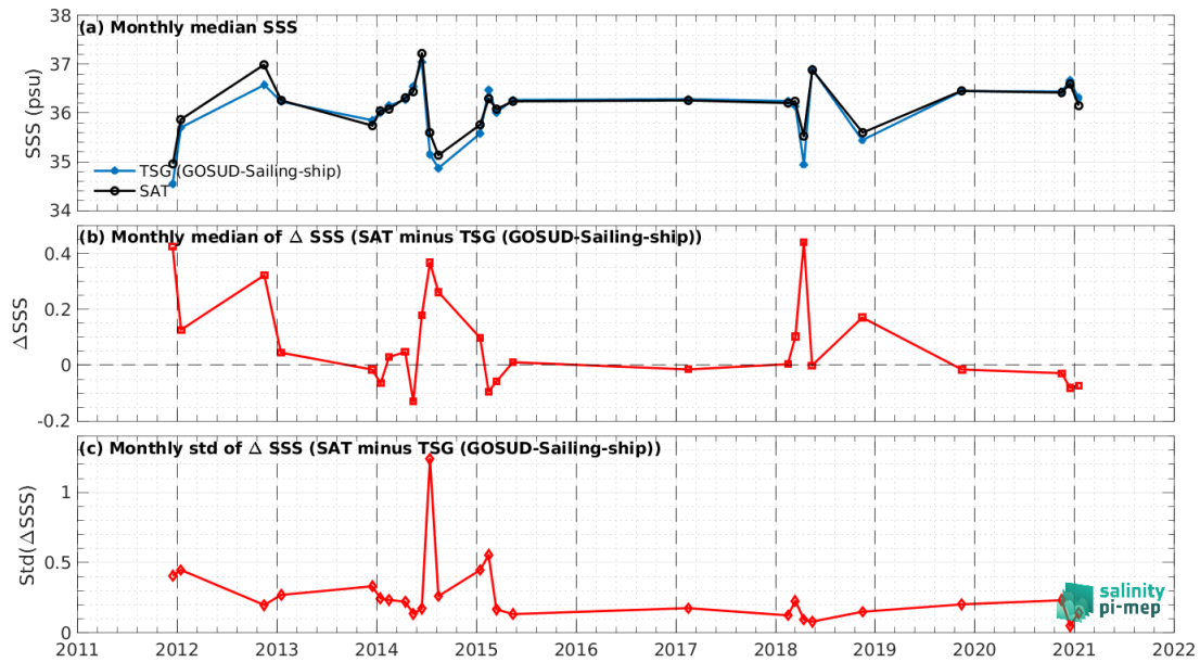
Figure 8: Time series of the monthly median SSS (top), median of \Delta SSS (Satellite - TSG (GOSUD-Sailing-ship)) and Std(\Delta SSS) (Satellite - TSG (GOSUD-Sailing-ship)) over the Tropical Atlantic Ocean Pi-MEP region considering all match-ups collected by the Pi-MEP.
