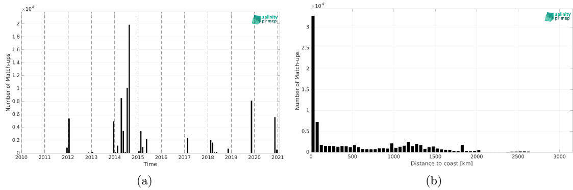
Figure 2: Number of match-ups between TSG (GOSUD-Sailing-ship) and SMAP SSS L4 OI v3 - Monthly (ESR) SSS as a function of time (a) and as function of the distance to coast (b) over the Tropical Atlantic Ocean Pi-MEP region and for the full satellite product period.
