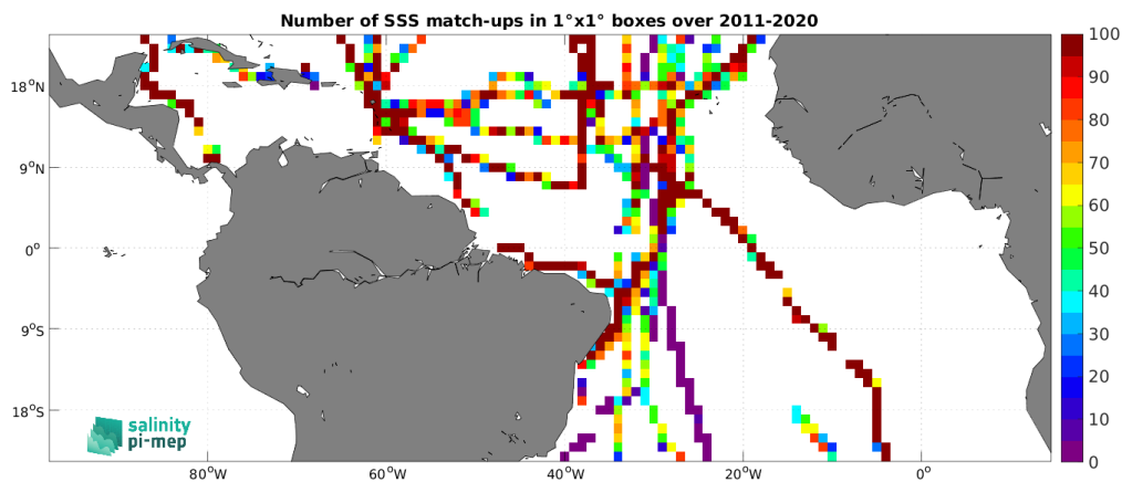
Figure 5: Number of SSS match-ups between TSG (GOSUD-Sailing-ship) SSS and the SMAP SSS L4 OI v3 - Monthly (ESR) SSS product for the Tropical Atlantic Ocean Pi-MEP region over 1^\circ \times 1^\circ boxes and for the full satellite product period.
