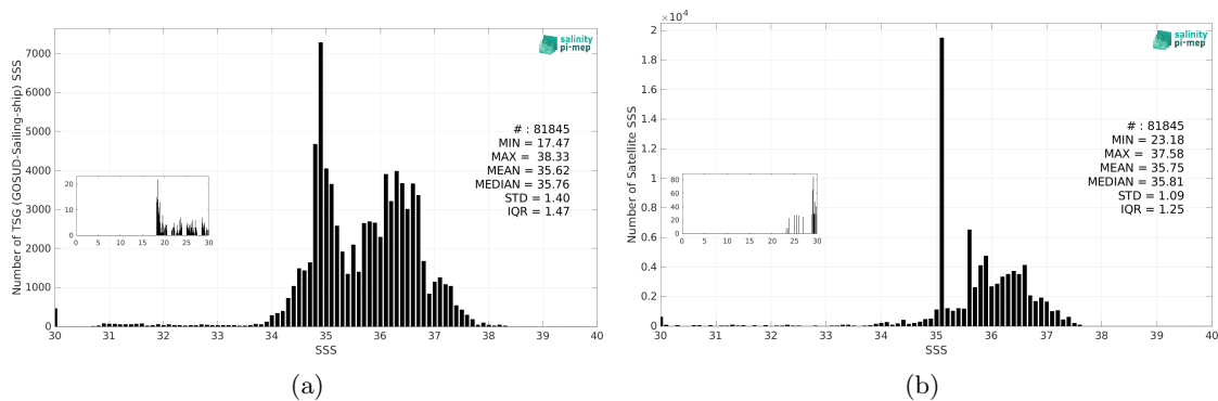
Figure 3: Histograms of SSS from TSG (GOSUD-Sailing-ship) (a) and SMAP SSS L4 OI v3 - Monthly (ESR) (b) considering all match-up pairs per bins of 0.1 over the Tropical Atlantic Ocean Pi-MEP region and for the full satellite product period.
